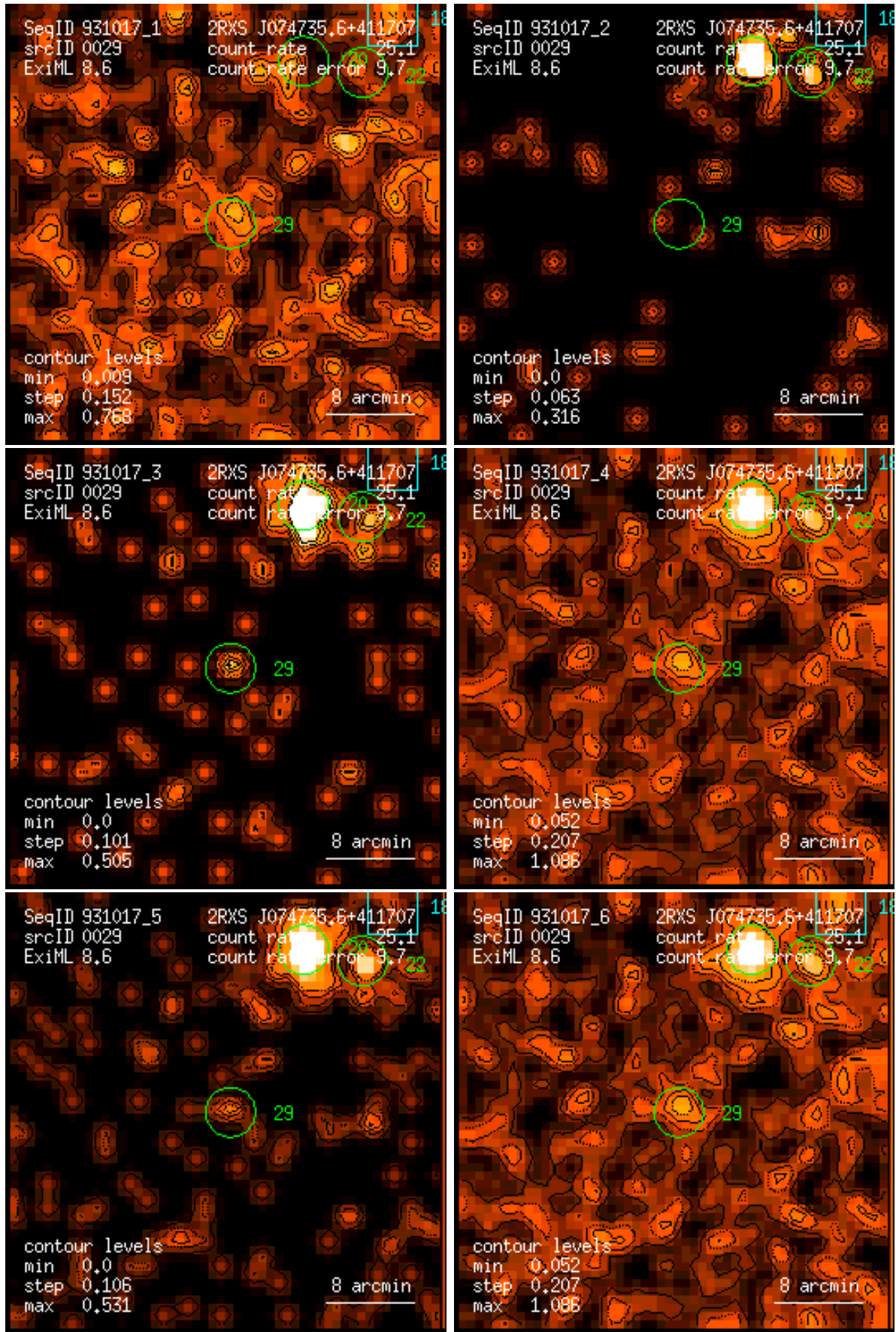
Figure 29: RASS 931017: detection 0029: band rate images, Gaussian filter: (1) PSPC channels 11 – 41, (2) 52 – 90, (3) 91 – 201, (4) 11 – 235, (5) 52 – 201, (6) 11 – 201. Broad band rates in counts/ks. Band rate contour levels in counts/ks/arcmin 2 .
