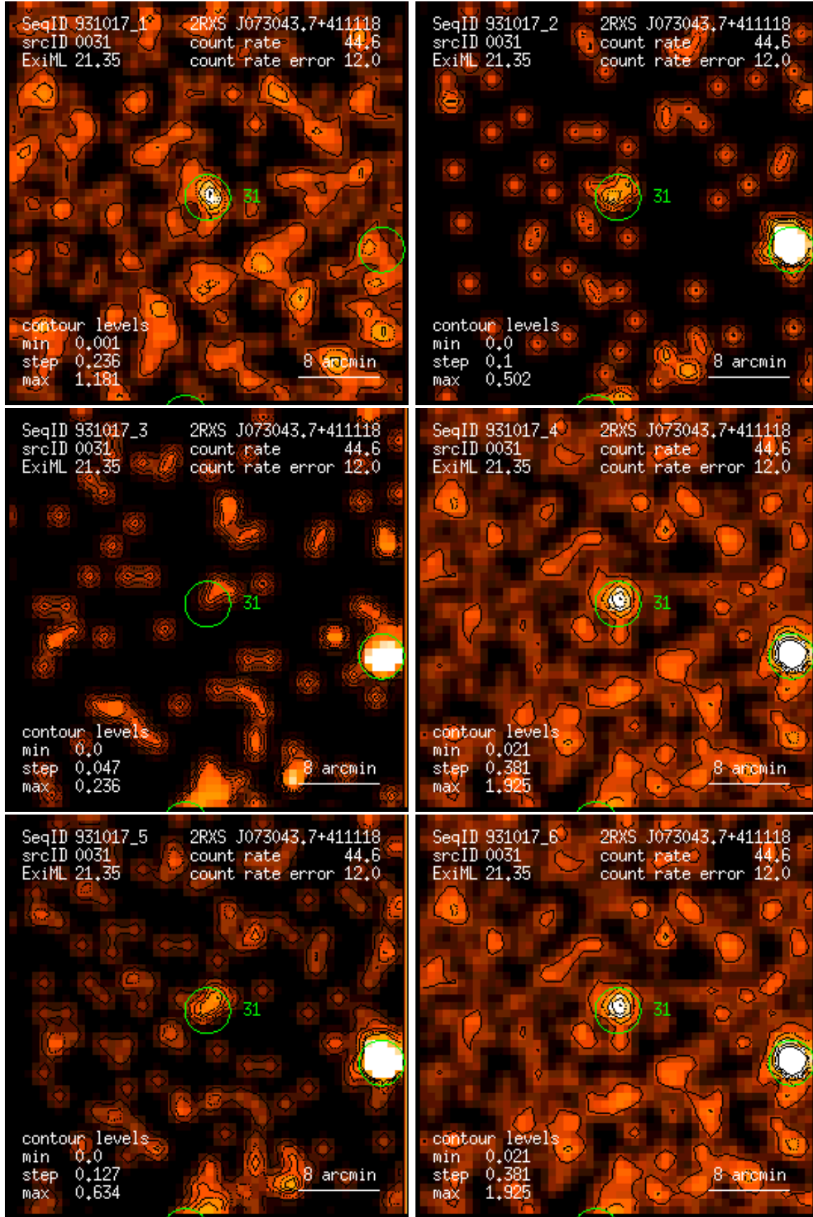
Figure 31: RASS 931017: detection 0031: band rate images, Gaussian filter: (1) PSPC channels 11 – 41, (2) 52 – 90, (3) 91 – 201, (4) 11 – 235, (5) 52 – 201, (6) 11 – 201. Broad band rates in counts/ks. Band rate contour levels in counts/ks/arcmin 2 .
