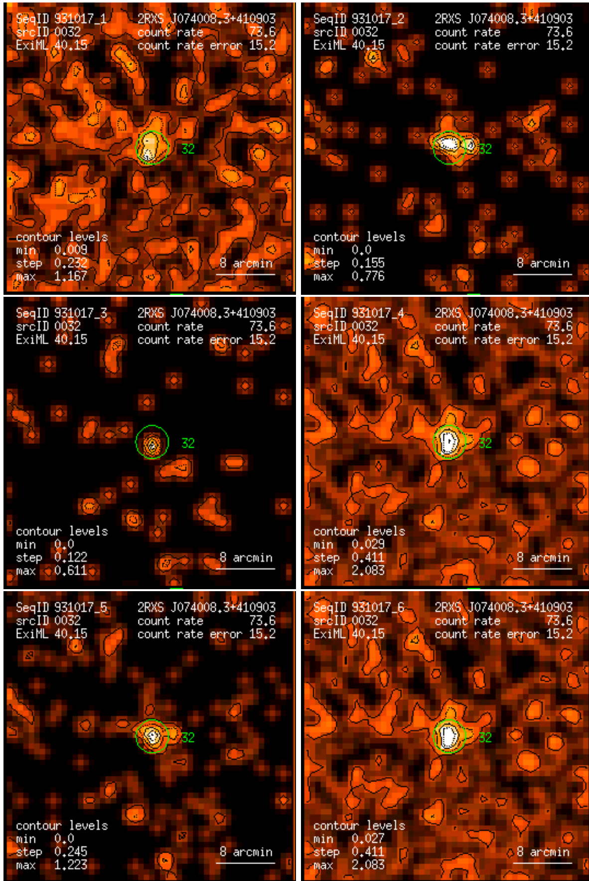
Figure 32: RASS 931017: detection 0032: band rate images, Gaussian filter: (1) PSPC channels 11 – 41, (2) 52 – 90, (3) 91 – 201, (4) 11 – 235, (5) 52 – 201, (6) 11 – 201. Broad band rates in counts/ks. Band rate contour levels in counts/ks/arcmin 2 .
