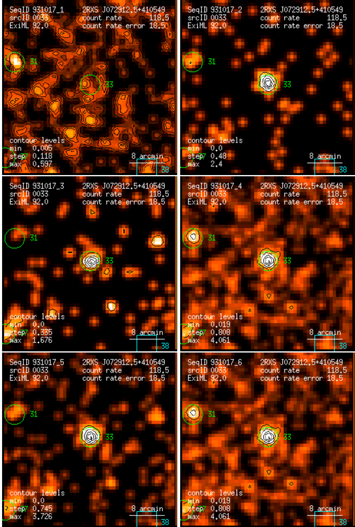
Figure 33: RASS 931017: detection 0033: band rate images, Gaussian filter: (1) PSPC channels 11 – 41, (2) 52 – 90, (3) 91 – 201, (4) 11 – 235, (5) 52 – 201, (6) 11 – 201. Broad band rates in counts/ks. Band rate contour levels in counts/ks/arcmin 2 .
