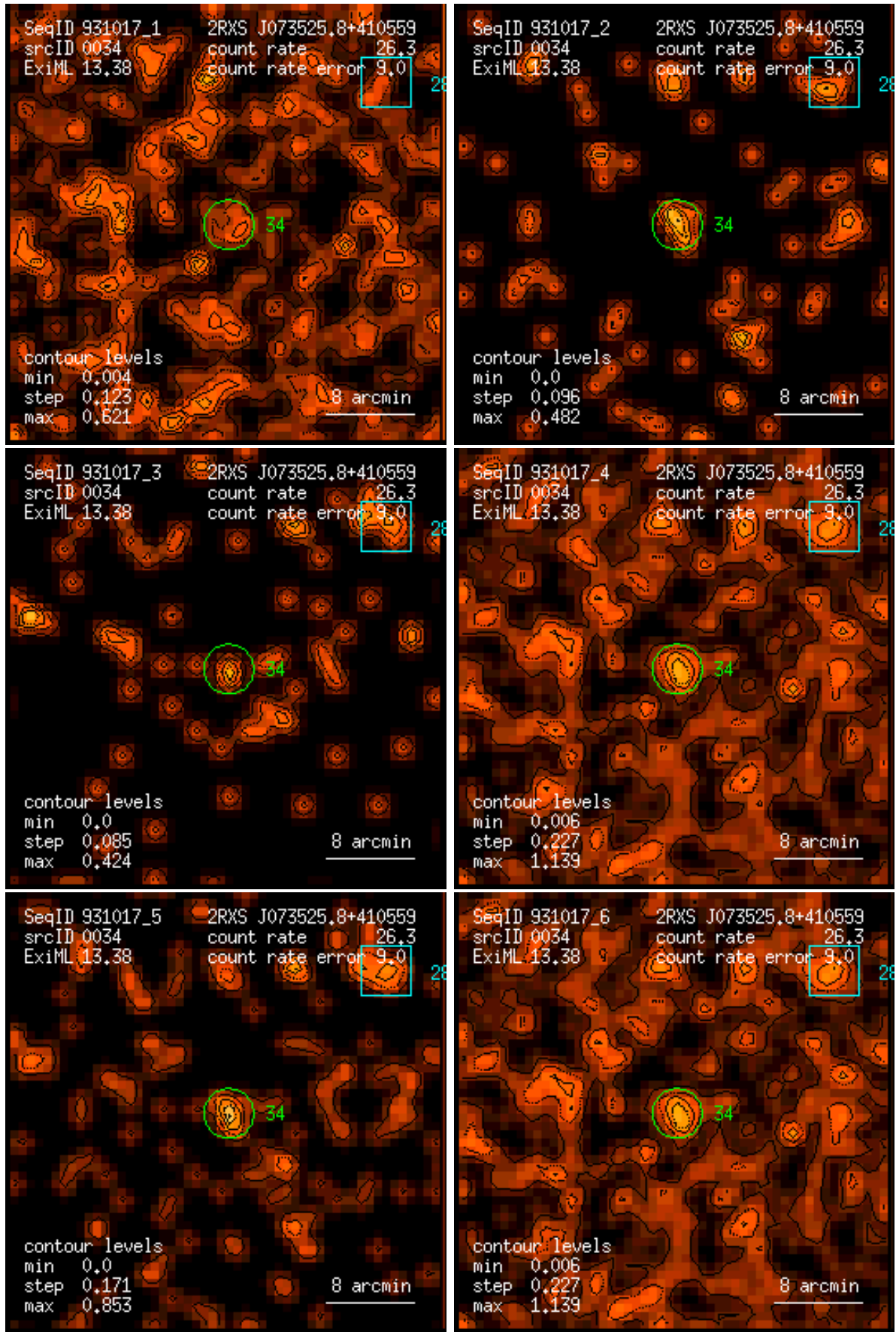
Figure 34: RASS 931017: detection 0034: band rate images, Gaussian filter: (1) PSPC channels 11 – 41, (2) 52 – 90, (3) 91 – 201, (4) 11 – 235, (5) 52 – 201, (6) 11 – 201. Broad band rates in counts/ks. Band rate contour levels in counts/ks/arcmin 2 .
