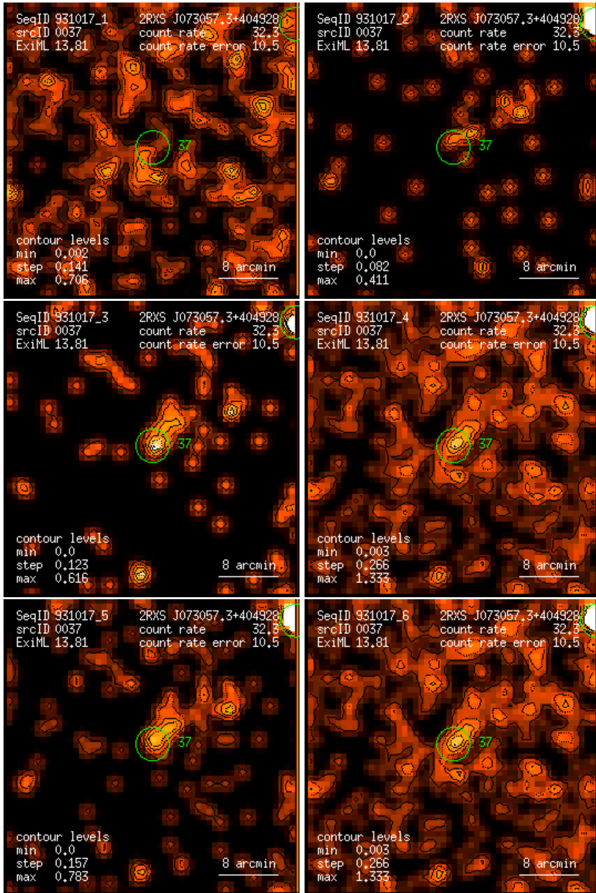
Figure 37: RASS 931017: detection 0037: band rate images, Gaussian filter: (1) PSPC channels 11 – 41, (2) 52 – 90, (3) 91 – 201, (4) 11 – 235, (5) 52 – 201, (6) 11 – 201. Broad band rates in counts/ks. Band rate contour levels in counts/ks/arcmin 2 .
