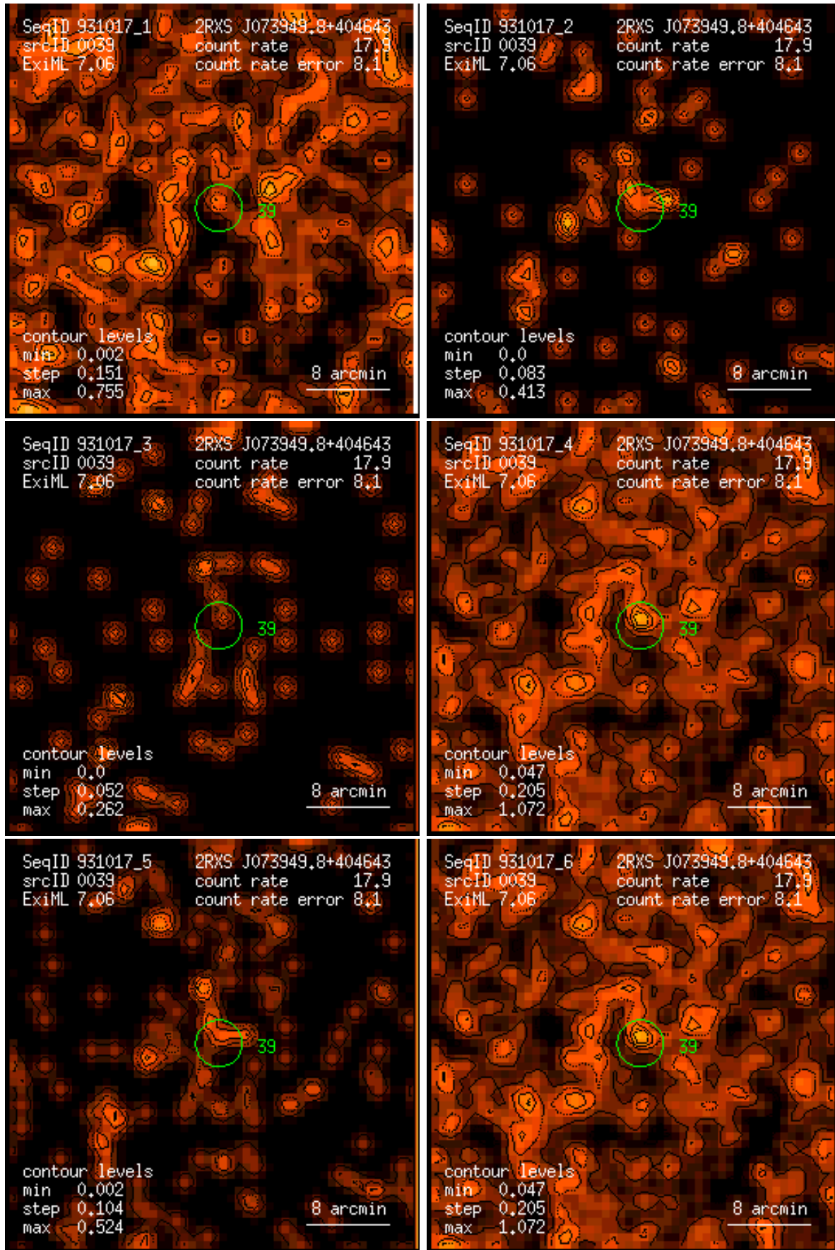
Figure 39: RASS 931017: detection 0039: band rate images, Gaussian filter: (1) PSPC channels 11 – 41, (2) 52 – 90, (3) 91 – 201, (4) 11 – 235, (5) 52 – 201, (6) 11 – 201. Broad band rates in counts/ks. Band rate contour levels in counts/ks/arcmin 2 .
