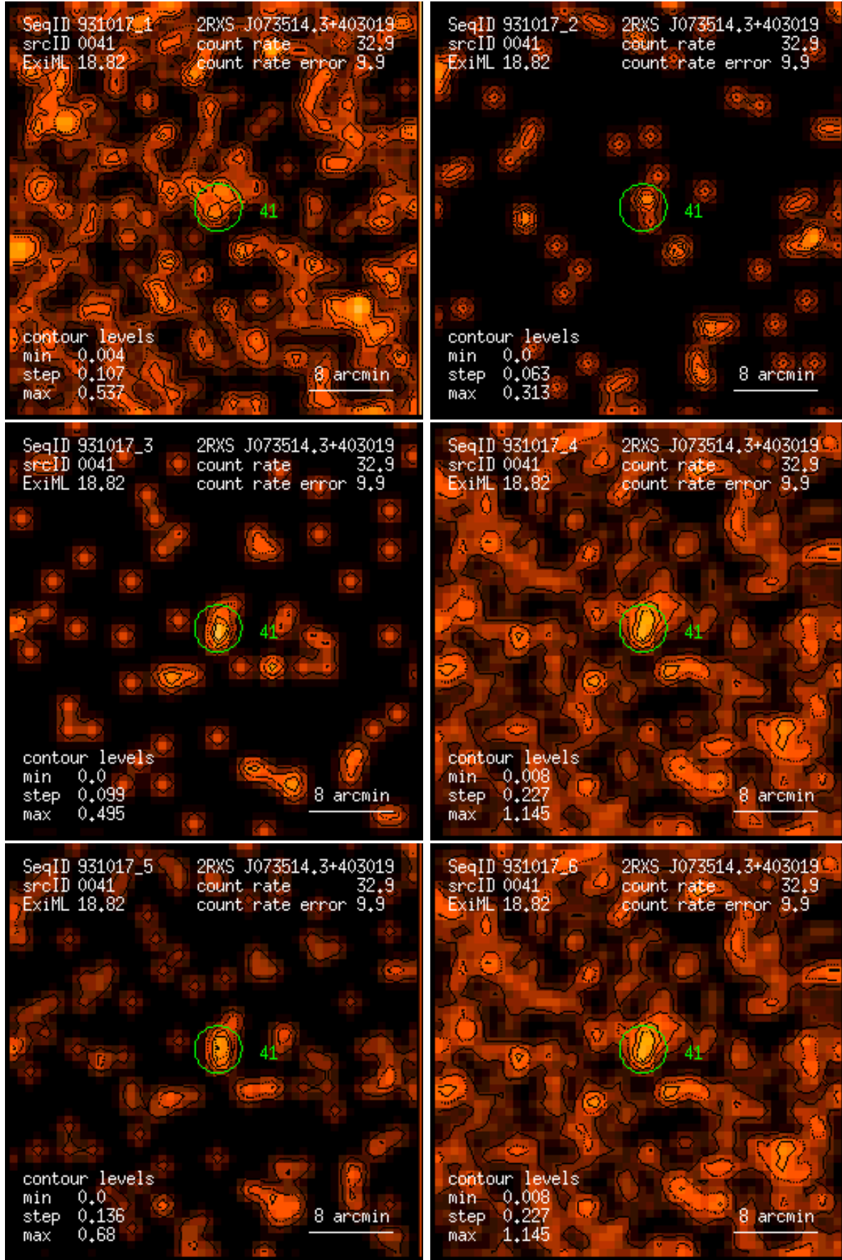
Figure 41: RASS 931017: detection 0041: band rate images, Gaussian filter: (1) PSPC channels 11 – 41, (2) 52 – 90, (3) 91 – 201, (4) 11 – 235, (5) 52 – 201, (6) 11 – 201. Broad band rates in counts/ks. Band rate contour levels in counts/ks/arcmin 2 .
