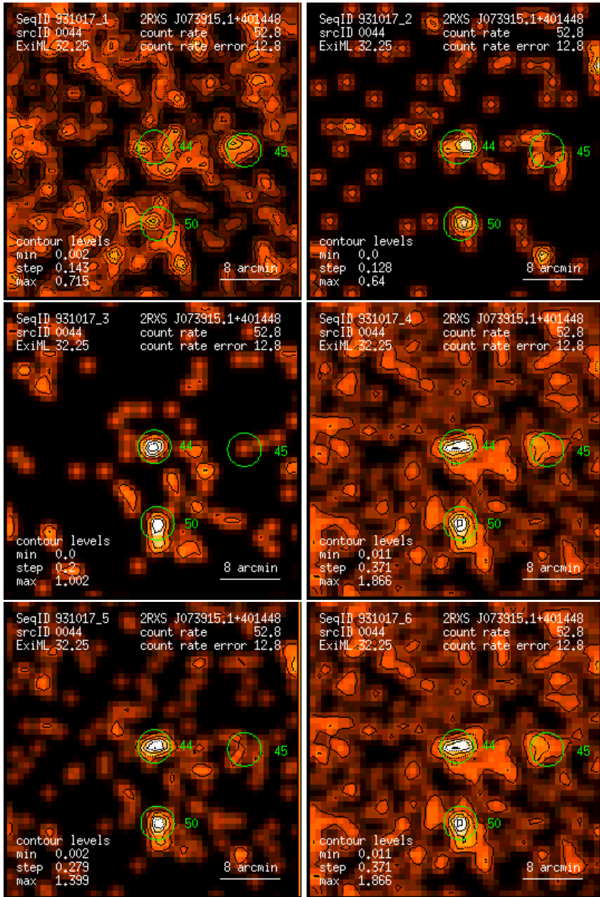
Figure 44: RASS 931017: detection 0044: band rate images, Gaussian filter: (1) PSPC channels 11 – 41, (2) 52 – 90, (3) 91 – 201, (4) 11 – 235, (5) 52 – 201, (6) 11 – 201. Broad band rates in counts/ks. Band rate contour levels in counts/ks/arcmin 2 .
