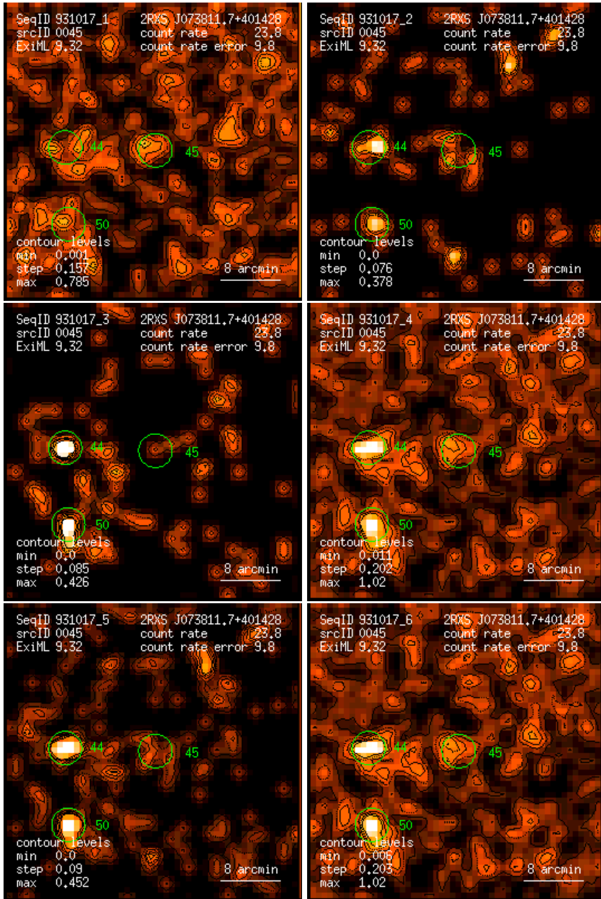
Figure 45: RASS 931017: detection 0045: band rate images, Gaussian filter: (1) PSPC channels 11 – 41, (2) 52 – 90, (3) 91 – 201, (4) 11 – 235, (5) 52 – 201, (6) 11 – 201. Broad band rates in counts/ks. Band rate contour levels in counts/ks/arcmin 2 .
