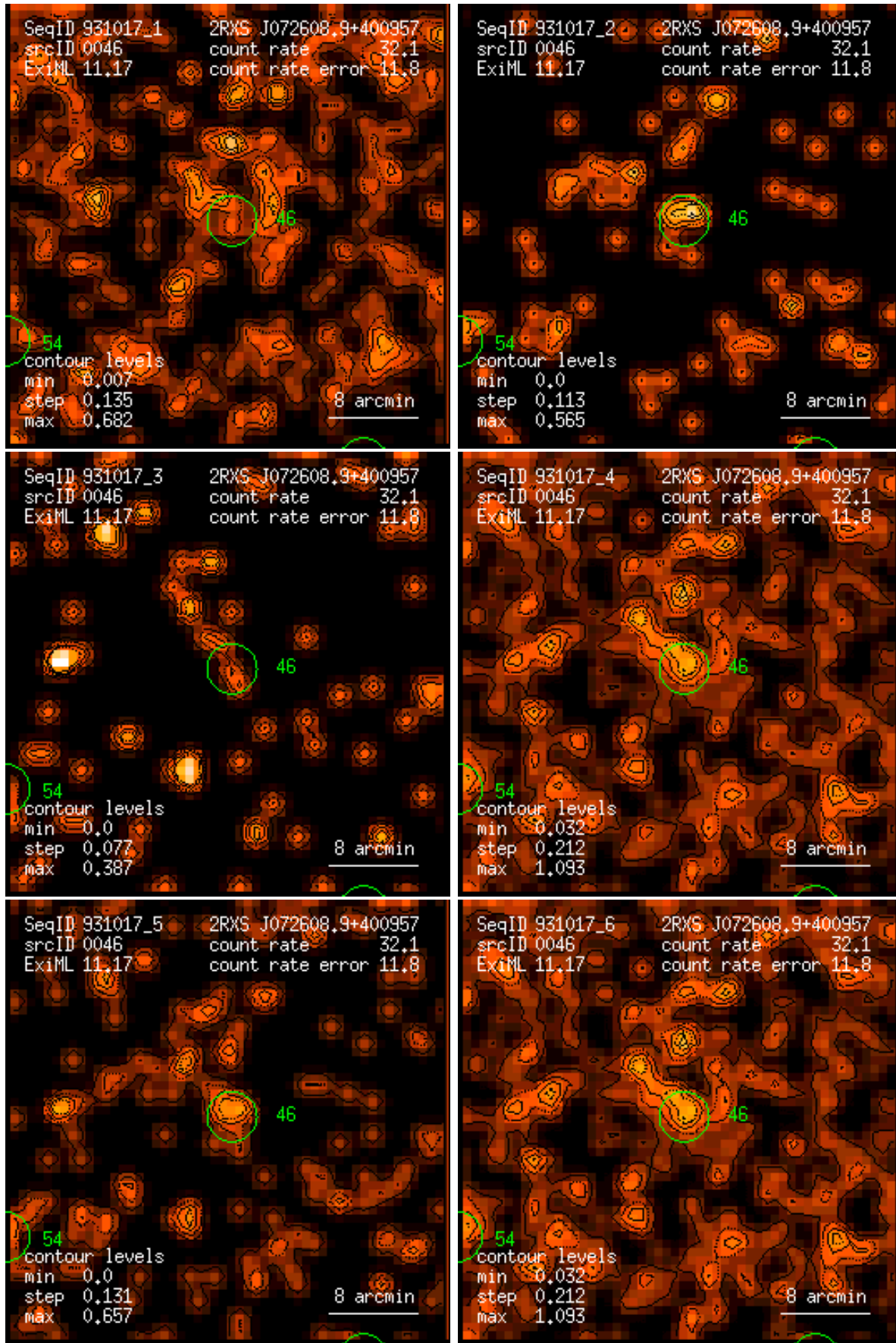
Figure 46: RASS 931017: detection 0046: band rate images, Gaussian filter: (1) PSPC channels 11 – 41, (2) 52 – 90, (3) 91 – 201, (4) 11 – 235, (5) 52 – 201, (6) 11 – 201. Broad band rates in counts/ks. Band rate contour levels in counts/ks/arcmin 2 .
