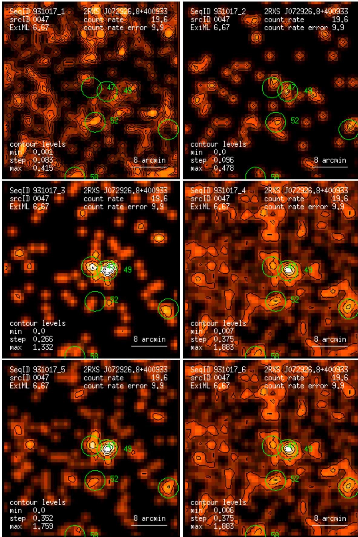
Figure 47: RASS 931017: detection 0047: band rate images, Gaussian filter: (1) PSPC channels 11 – 41, (2) 52 – 90, (3) 91 – 201, (4) 11 – 235, (5) 52 – 201, (6) 11 – 201. Broad band rates in counts/ks. Band rate contour levels in counts/ks/arcmin 2 .
