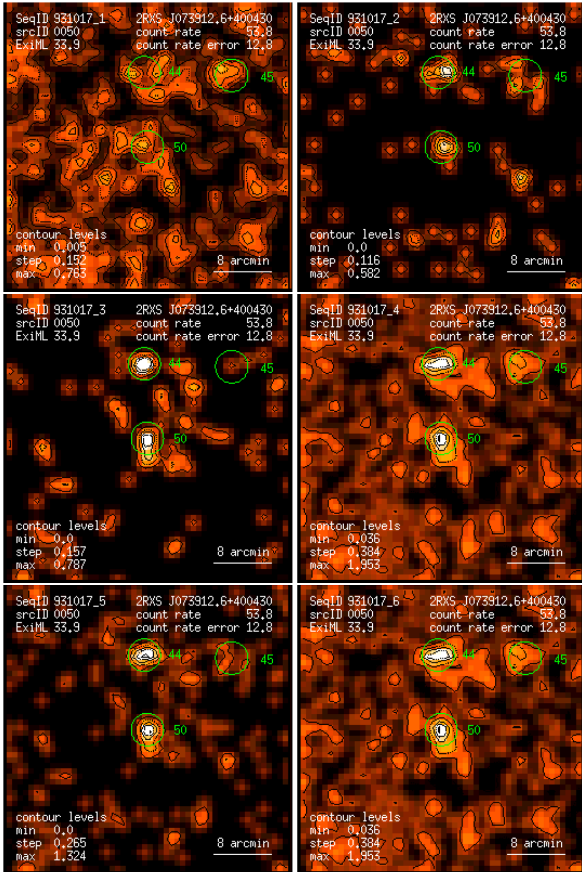
Figure 50: RASS 931017: detection 0050: band rate images, Gaussian filter: (1) PSPC channels 11 – 41, (2) 52 – 90, (3) 91 – 201, (4) 11 – 235, (5) 52 – 201, (6) 11 – 201. Broad band rates in counts/ks. Band rate contour levels in counts/ks/arcmin 2 .
