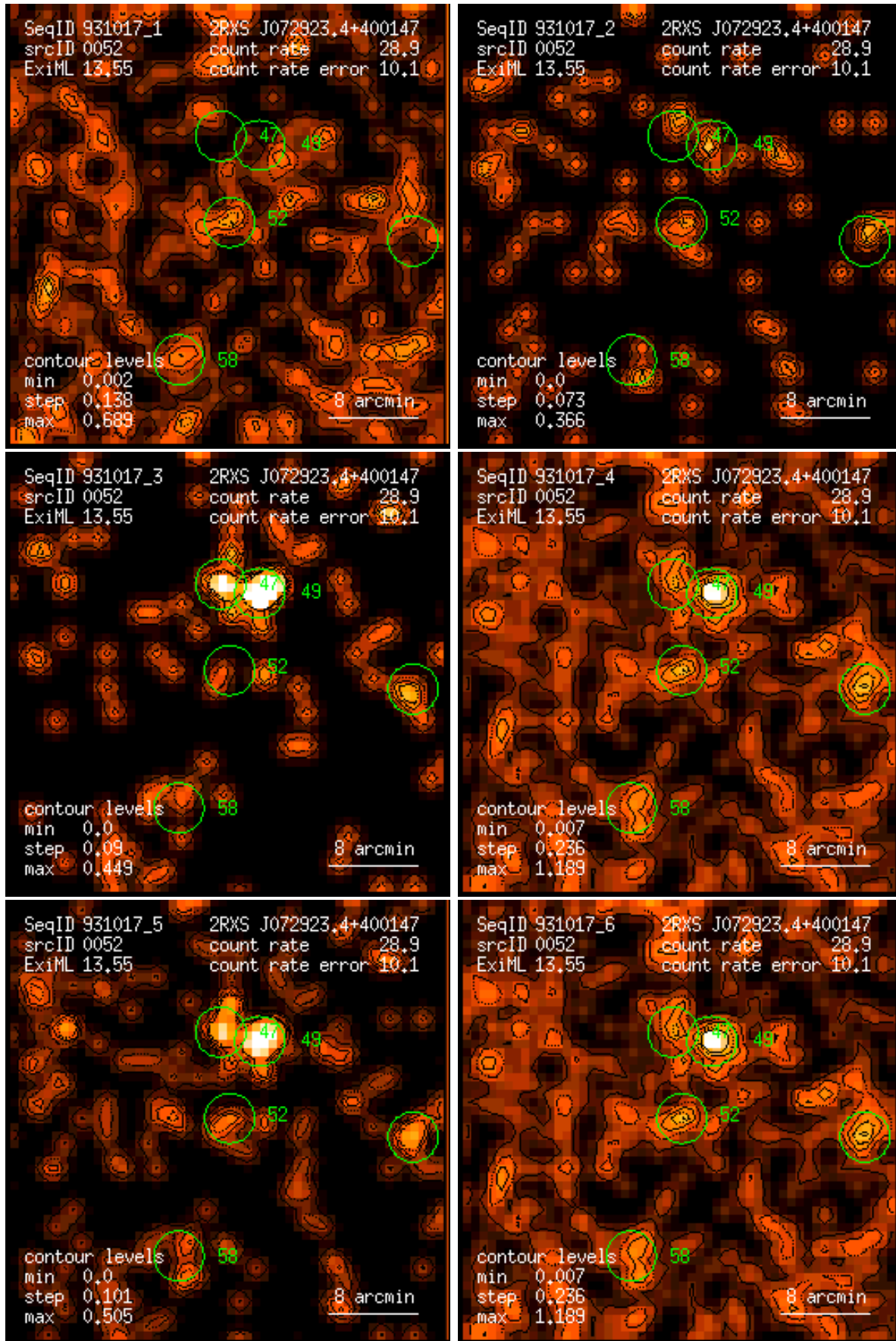
Figure 52: RASS 931017: detection 0052: band rate images, Gaussian filter: (1) PSPC channels 11 – 41, (2) 52 – 90, (3) 91 – 201, (4) 11 – 235, (5) 52 – 201, (6) 11 – 201. Broad band rates in counts/ks. Band rate contour levels in counts/ks/arcmin 2 .
