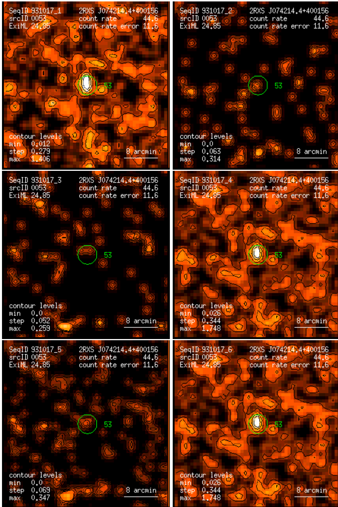
Figure 53: RASS 931017: detection 0053: band rate images, Gaussian filter: (1) PSPC channels 11 – 41, (2) 52 – 90, (3) 91 – 201, (4) 11 – 235, (5) 52 – 201, (6) 11 – 201. Broad band rates in counts/ks. Band rate contour levels in counts/ks/arcmin 2 .
