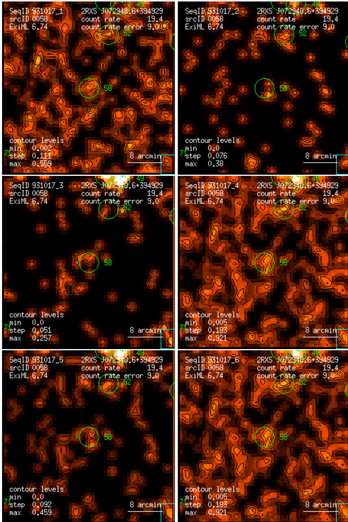
Figure 58: RASS 931017: detection 0058: band rate images, Gaussian filter: (1) PSPC channels 11 – 41, (2) 52 – 90, (3) 91 – 201, (4) 11 – 235, (5) 52 – 201, (6) 11 – 201. Broad band rates in counts/ks. Band rate contour levels in counts/ks/arcmin 2 .
