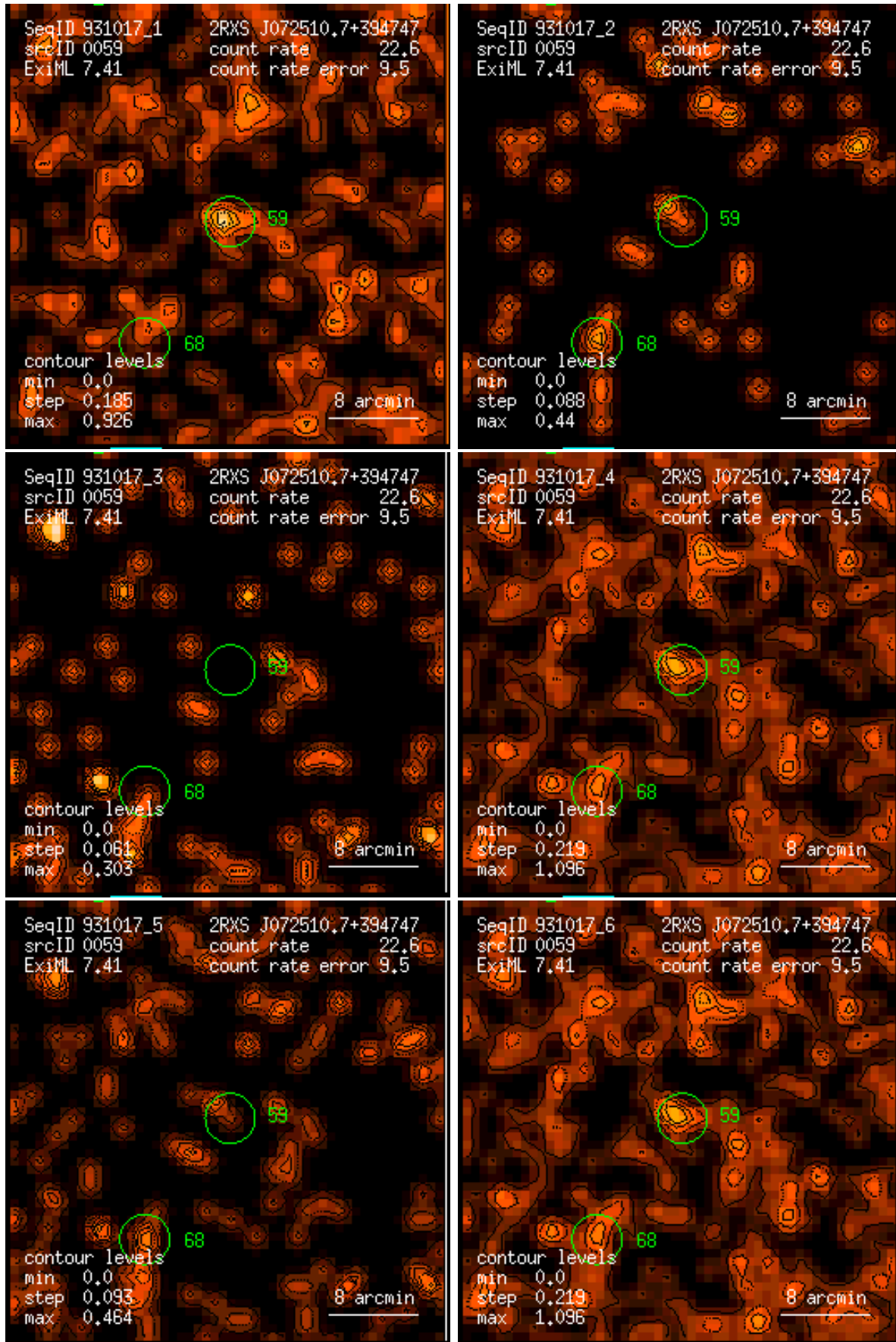
Figure 59: RASS 931017: detection 0059: band rate images, Gaussian filter: (1) PSPC channels 11 – 41, (2) 52 – 90, (3) 91 – 201, (4) 11 – 235, (5) 52 – 201, (6) 11 – 201. Broad band rates in counts/ks. Band rate contour levels in counts/ks/arcmin 2 .
