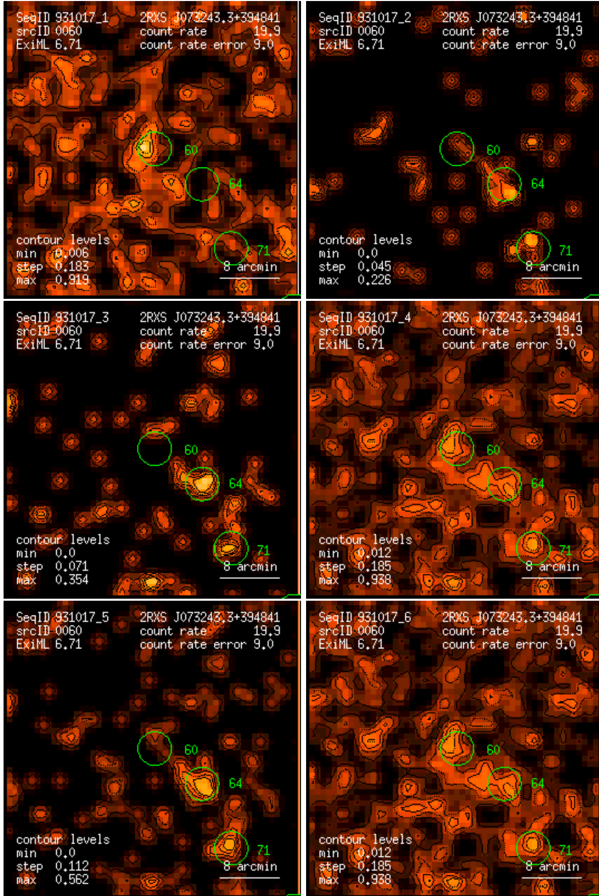
Figure 60: RASS 931017: detection 0060: band rate images, Gaussian filter: (1) PSPC channels 11 – 41, (2) 52 – 90, (3) 91 – 201, (4) 11 – 235, (5) 52 – 201, (6) 11 – 201. Broad band rates in counts/ks. Band rate contour levels in counts/ks/arcmin 2 .
