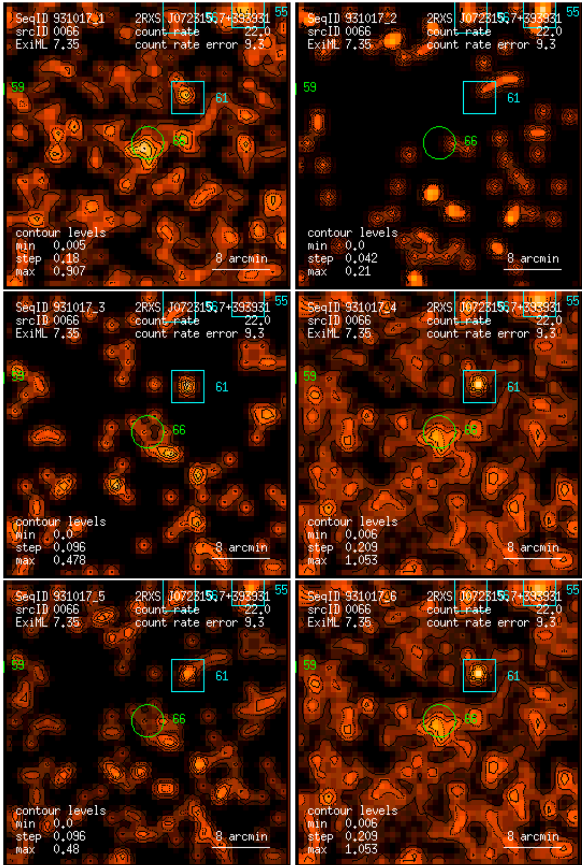
Figure 66: RASS 931017: detection 0066: band rate images, Gaussian filter: (1) PSPC channels 11 – 41, (2) 52 – 90, (3) 91 – 201, (4) 11 – 235, (5) 52 – 201, (6) 11 – 201. Broad band rates in counts/ks. Band rate contour levels in counts/ks/arcmin 2 .
