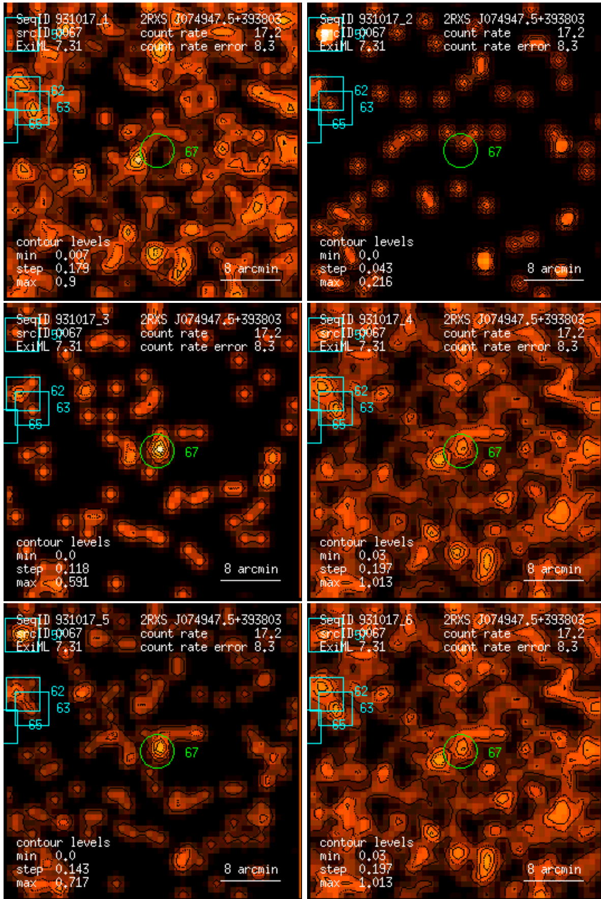
Figure 67: RASS 931017: detection 0067: band rate images, Gaussian filter: (1) PSPC channels 11 – 41, (2) 52 – 90, (3) 91 – 201, (4) 11 – 235, (5) 52 – 201, (6) 11 – 201. Broad band rates in counts/ks. Band rate contour levels in counts/ks/arcmin 2 .
