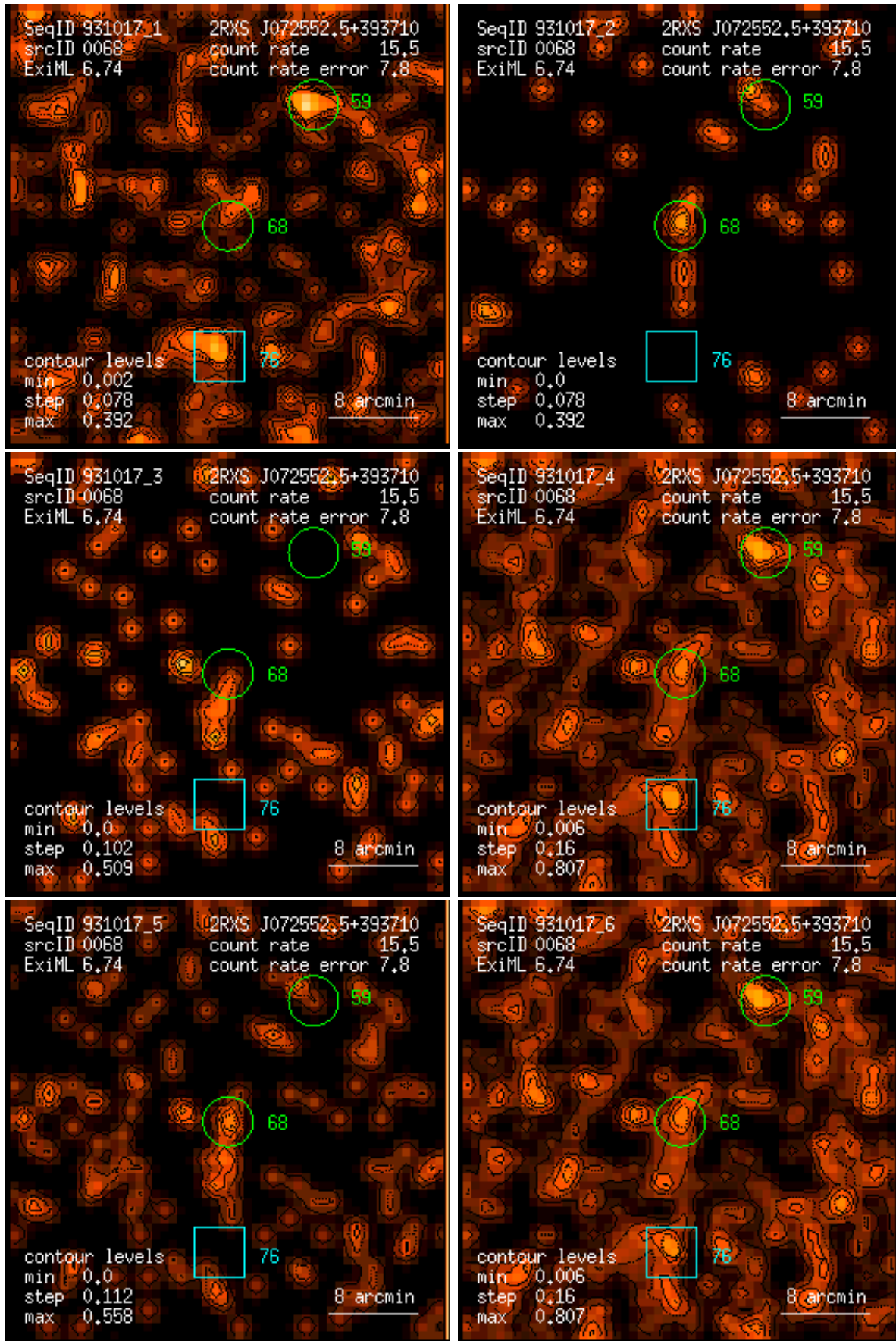
Figure 68: RASS 931017: detection 0068: band rate images, Gaussian filter: (1) PSPC channels 11 – 41, (2) 52 – 90, (3) 91 – 201, (4) 11 – 235, (5) 52 – 201, (6) 11 – 201. Broad band rates in counts/ks. Band rate contour levels in counts/ks/arcmin 2 .
