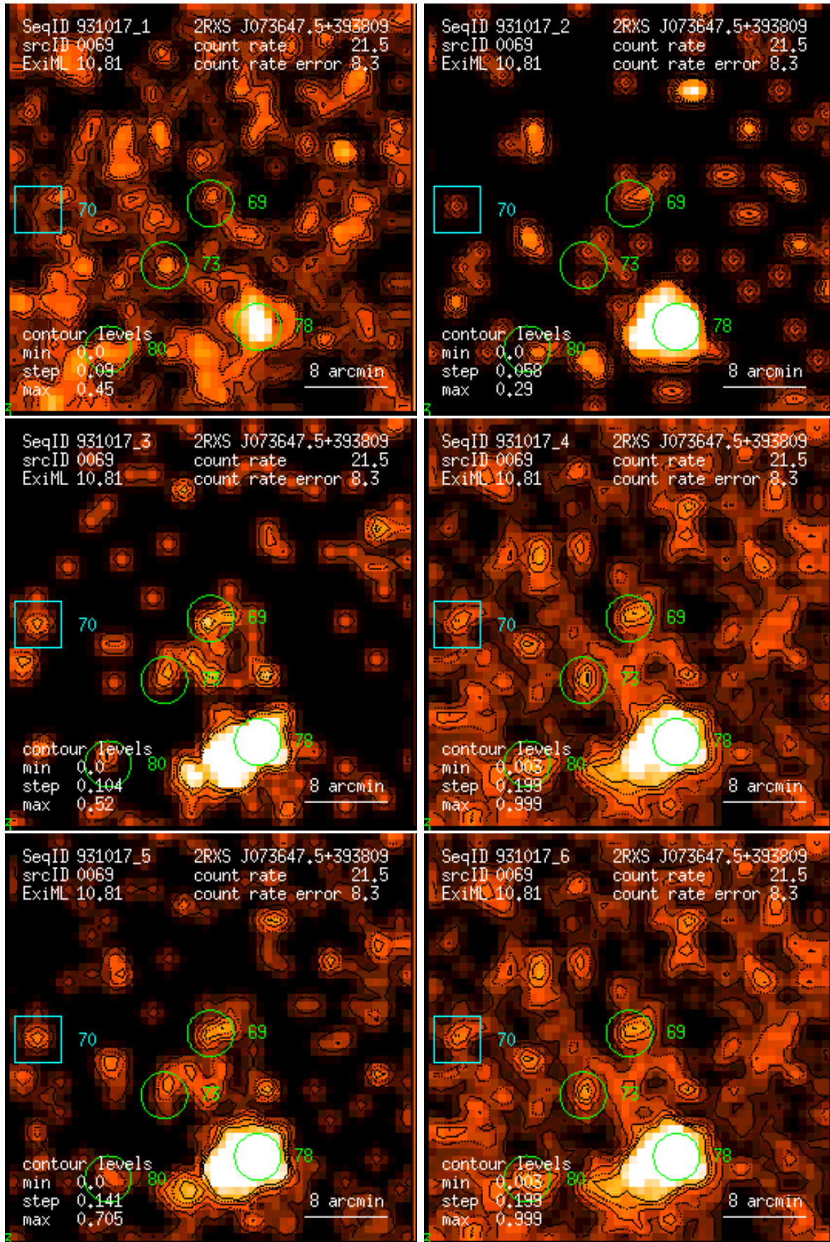
Figure 69: RASS 931017: detection 0069: band rate images, Gaussian filter: (1) PSPC channels 11 – 41, (2) 52 – 90, (3) 91 – 201, (4) 11 – 235, (5) 52 – 201, (6) 11 – 201. Broad band rates in counts/ks. Band rate contour levels in counts/ks/arcmin 2 .
