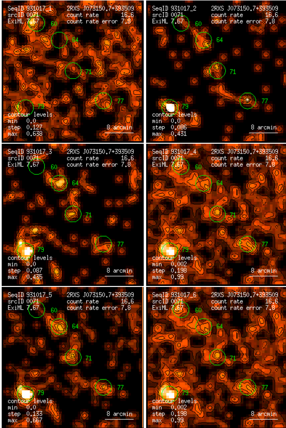
Figure 71: RASS 931017: detection 0071: band rate images, Gaussian filter: (1) PSPC channels 11 – 41, (2) 52 – 90, (3) 91 – 201, (4) 11 – 235, (5) 52 – 201, (6) 11 – 201. Broad band rates in counts/ks. Band rate contour levels in counts/ks/arcmin 2 .
