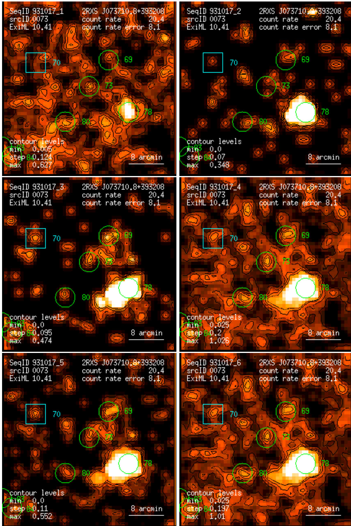
Figure 73: RASS 931017: detection 0073: band rate images, Gaussian filter: (1) PSPC channels 11 – 41, (2) 52 – 90, (3) 91 – 201, (4) 11 – 235, (5) 52 – 201, (6) 11 – 201. Broad band rates in counts/ks. Band rate contour levels in counts/ks/arcmin 2 .
