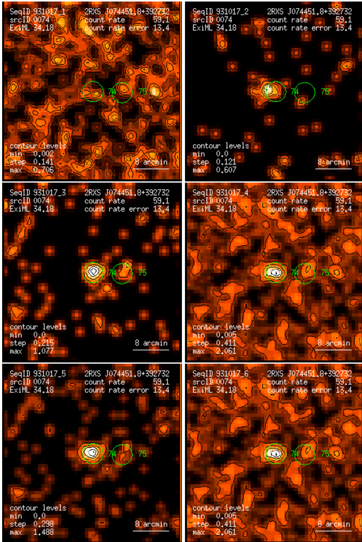
Figure 74: RASS 931017: detection 0074: band rate images, Gaussian filter: (1) PSPC channels 11 – 41, (2) 52 – 90, (3) 91 – 201, (4) 11 – 235, (5) 52 – 201, (6) 11 – 201. Broad band rates in counts/ks. Band rate contour levels in counts/ks/arcmin 2 .
