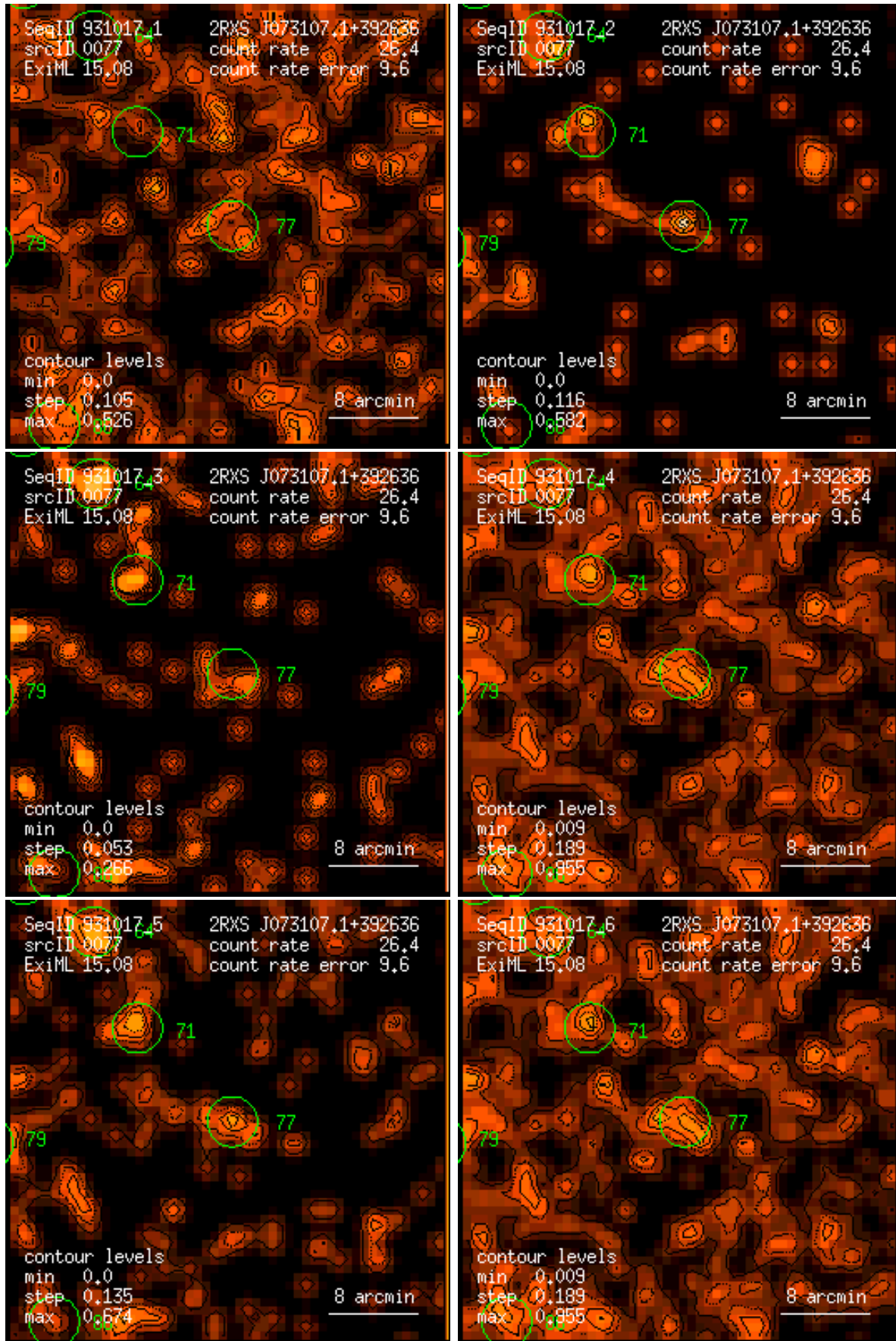
Figure 77: RASS 931017: detection 0077: band rate images, Gaussian filter: (1) PSPC channels 11 – 41, (2) 52 – 90, (3) 91 – 201, (4) 11 – 235, (5) 52 – 201, (6) 11 – 201. Broad band rates in counts/ks. Band rate contour levels in counts/ks/arcmin 2 .
