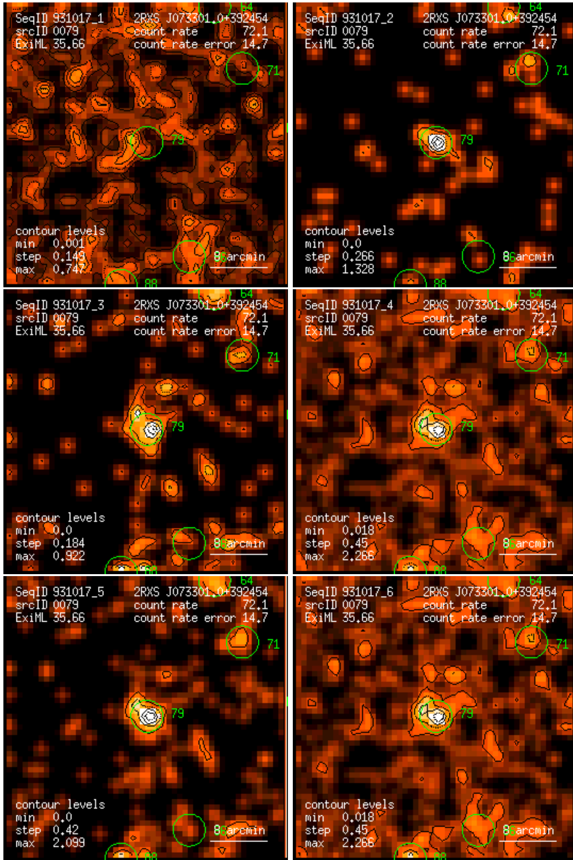
Figure 79: RASS 931017: detection 0079: band rate images, Gaussian filter: (1) PSPC channels 11 – 41, (2) 52 – 90, (3) 91 – 201, (4) 11 – 235, (5) 52 – 201, (6) 11 – 201. Broad band rates in counts/ks. Band rate contour levels in counts/ks/arcmin 2 .
