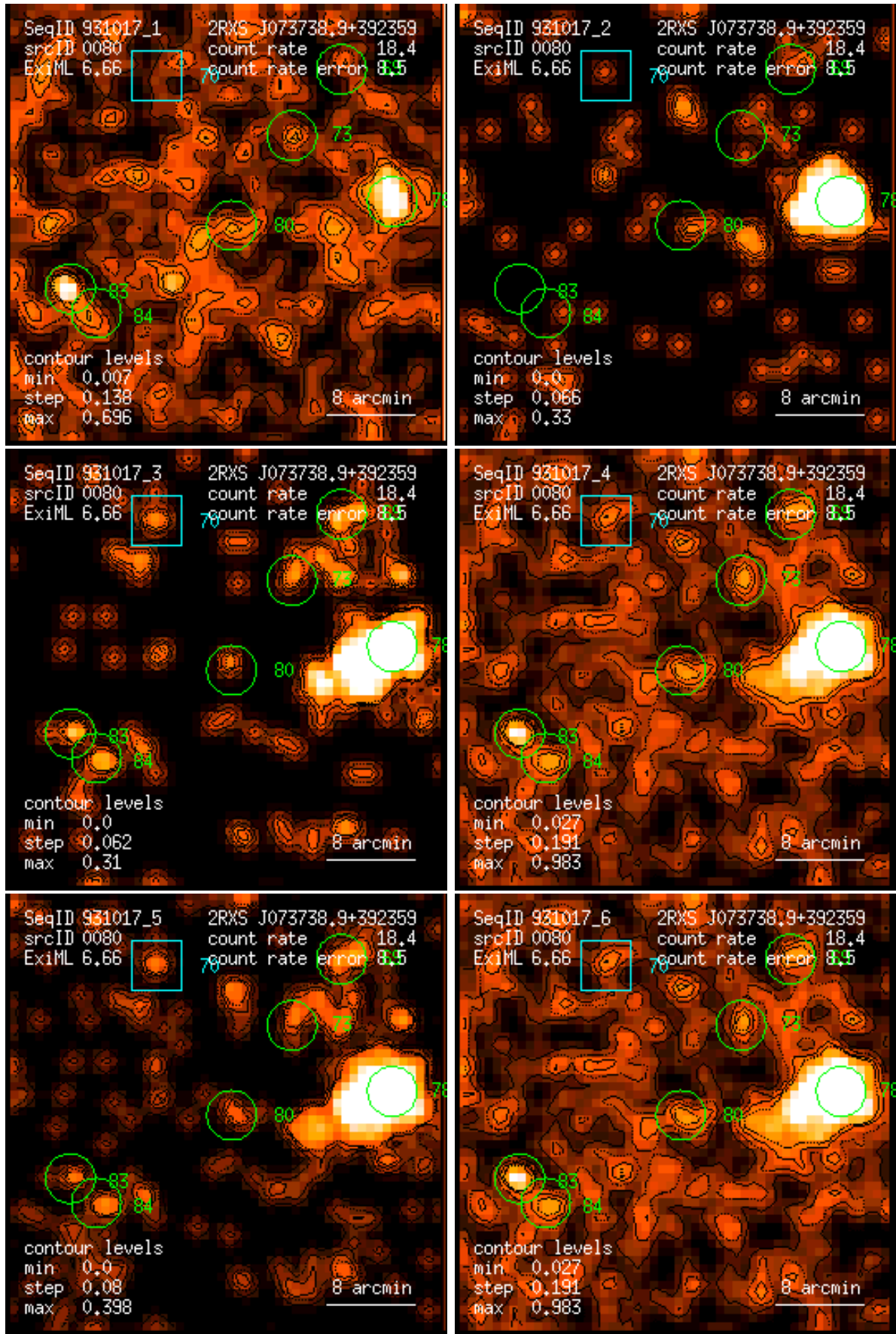
Figure 80: RASS 931017: detection 0080: band rate images, Gaussian filter: (1) PSPC channels 11 – 41, (2) 52 – 90, (3) 91 – 201, (4) 11 – 235, (5) 52 – 201, (6) 11 – 201. Broad band rates in counts/ks. Band rate contour levels in counts/ks/arcmin 2 .
