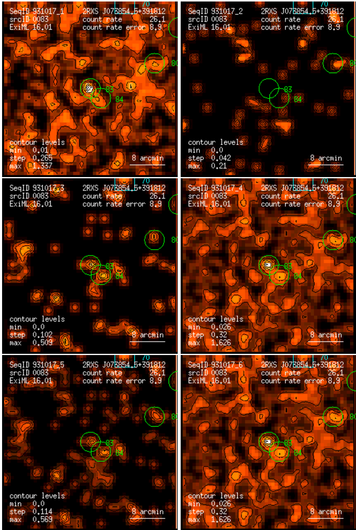
Figure 83: RASS 931017: detection 0083: band rate images, Gaussian filter: (1) PSPC channels 11 – 41, (2) 52 – 90, (3) 91 – 201, (4) 11 – 235, (5) 52 – 201, (6) 11 – 201. Broad band rates in counts/ks. Band rate contour levels in counts/ks/arcmin 2 .
