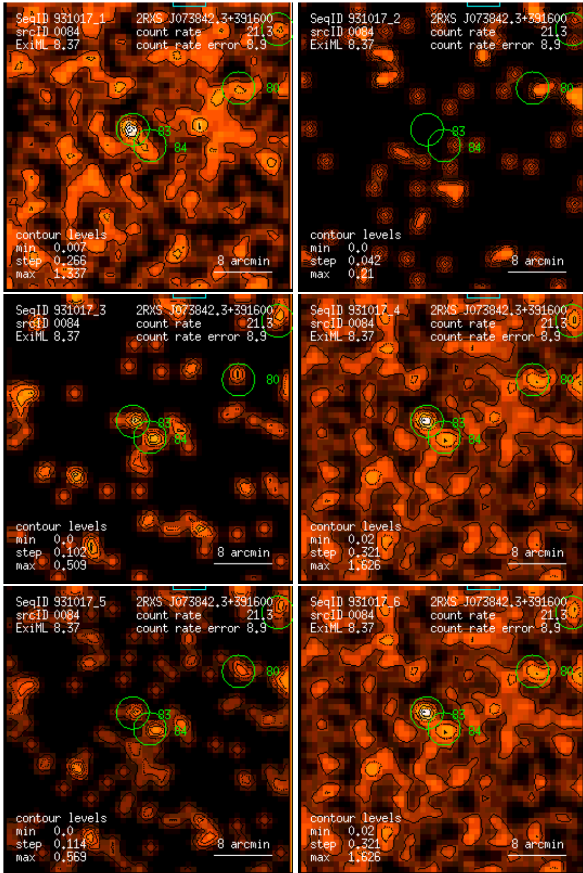
Figure 84: RASS 931017: detection 0084: band rate images, Gaussian filter: (1) PSPC channels 11 – 41, (2) 52 – 90, (3) 91 – 201, (4) 11 – 235, (5) 52 – 201, (6) 11 – 201. Broad band rates in counts/ks. Band rate contour levels in counts/ks/arcmin 2 .
