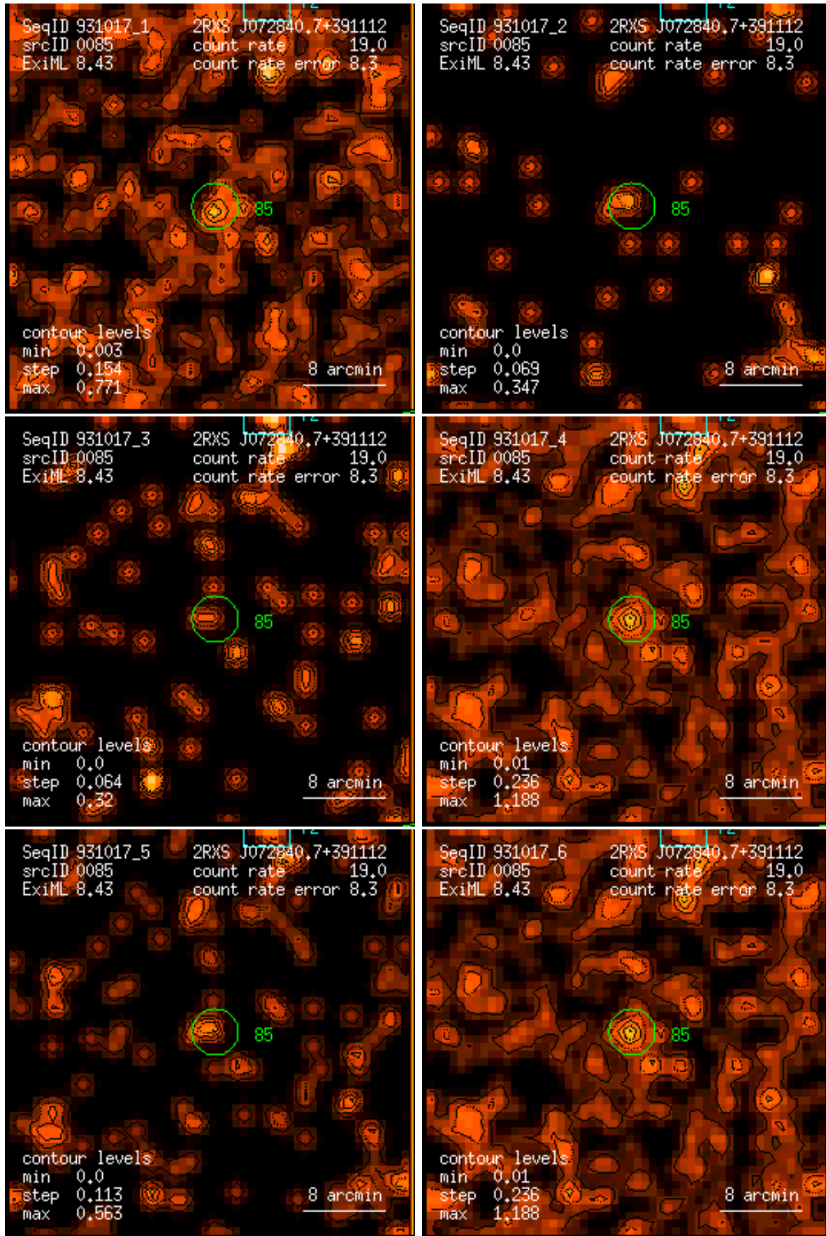
Figure 85: RASS 931017: detection 0085: band rate images, Gaussian filter: (1) PSPC channels 11 – 41, (2) 52 – 90, (3) 91 – 201, (4) 11 – 235, (5) 52 – 201, (6) 11 – 201. Broad band rates in counts/ks. Band rate contour levels in counts/ks/arcmin 2 .
