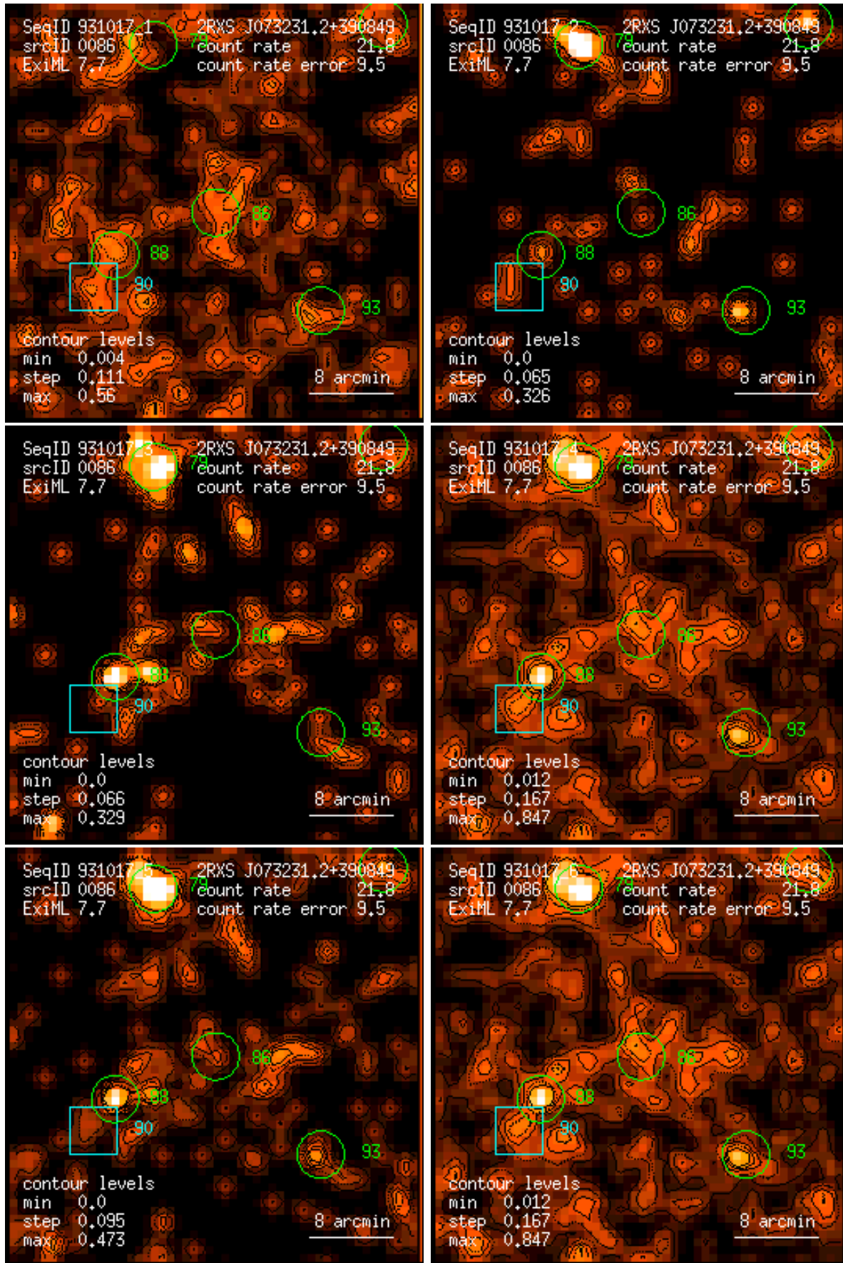
Figure 86: RASS 931017: detection 0086: band rate images, Gaussian filter: (1) PSPC channels 11 – 41, (2) 52 – 90, (3) 91 – 201, (4) 11 – 235, (5) 52 – 201, (6) 11 – 201. Broad band rates in counts/ks. Band rate contour levels in counts/ks/arcmin 2 .
