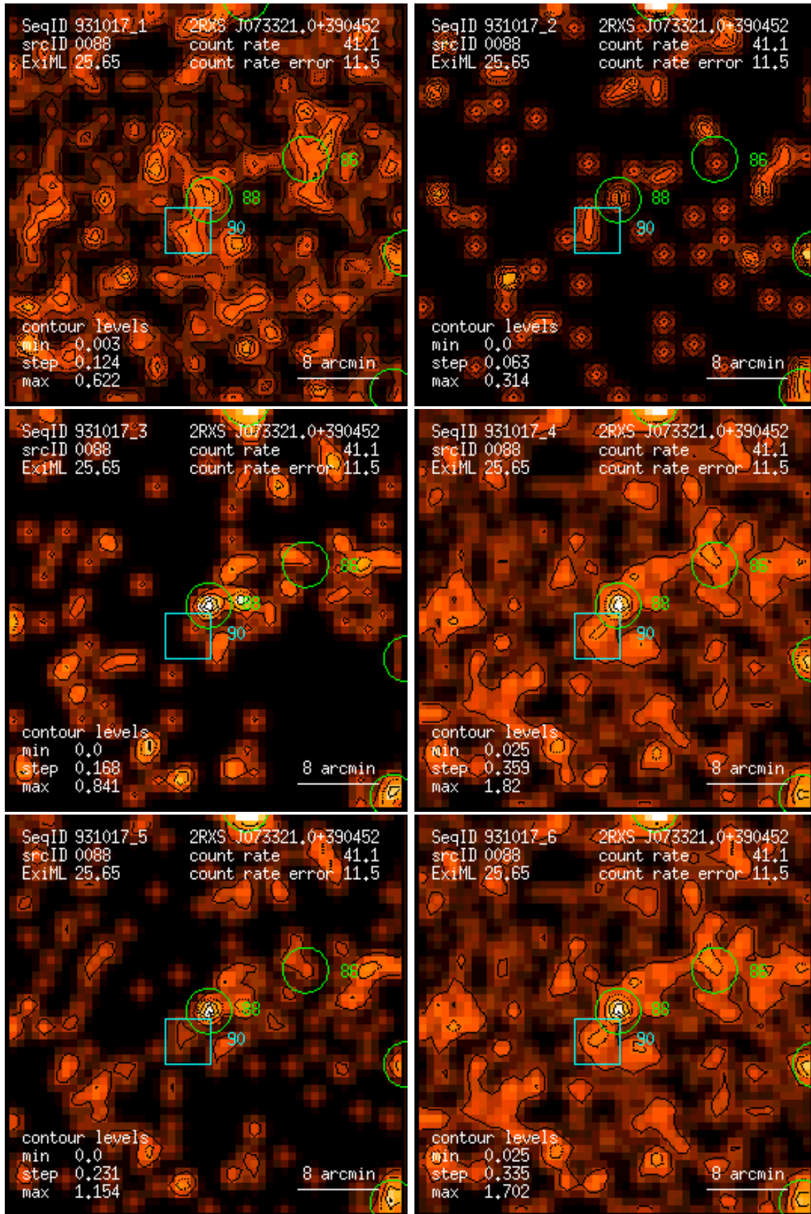
Figure 88: RASS 931017: detection 0088: band rate images, Gaussian filter: (1) PSPC channels 11 – 41, (2) 52 – 90, (3) 91 – 201, (4) 11 – 235, (5) 52 – 201, (6) 11 – 201. Broad band rates in counts/ks. Band rate contour levels in counts/ks/arcmin 2 .
