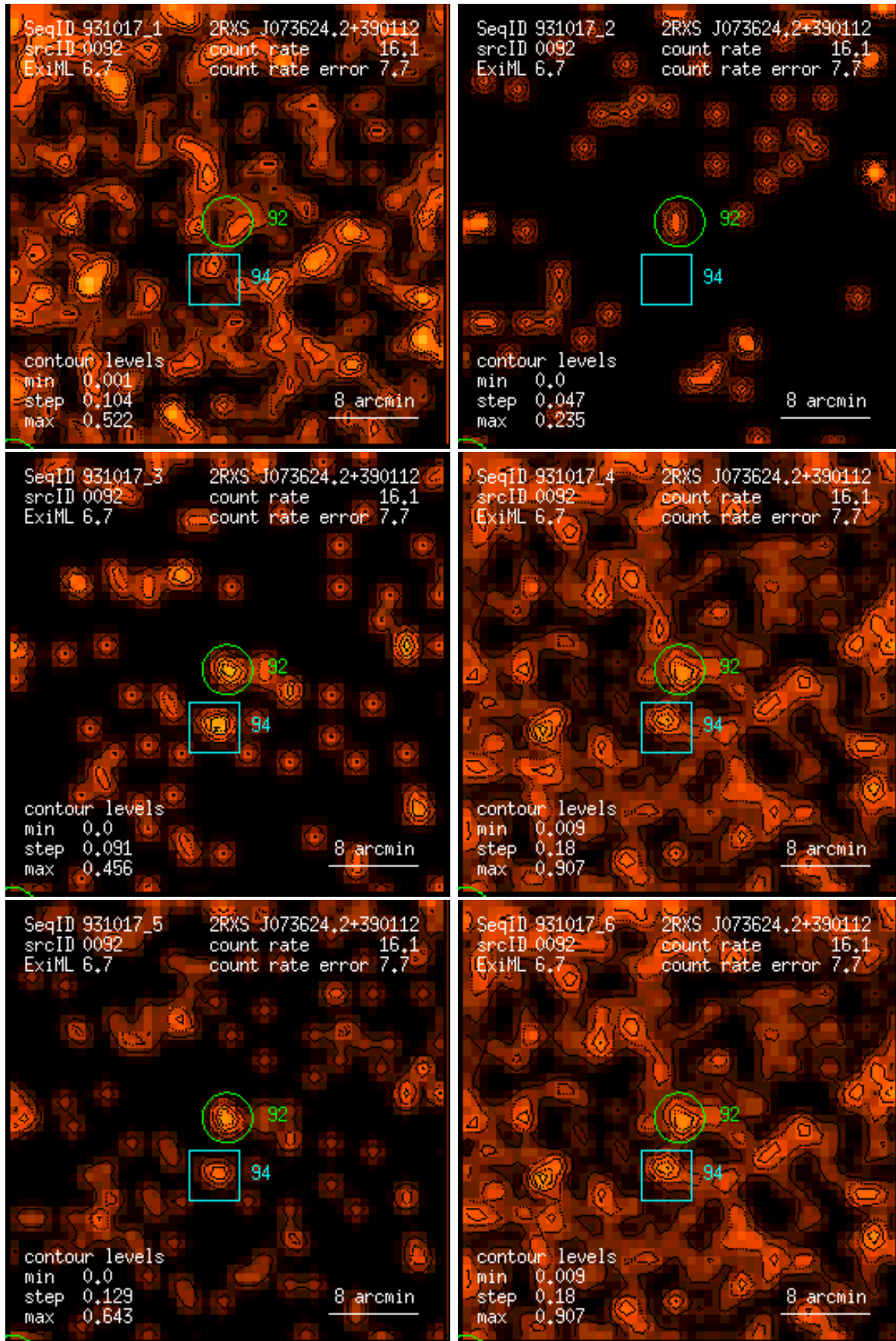
Figure 92: RASS 931017: detection 0092: band rate images, Gaussian filter: (1) PSPC channels 11 – 41, (2) 52 – 90, (3) 91 – 201, (4) 11 – 235, (5) 52 – 201, (6) 11 – 201. Broad band rates in counts/ks. Band rate contour levels in counts/ks/arcmin 2 .
