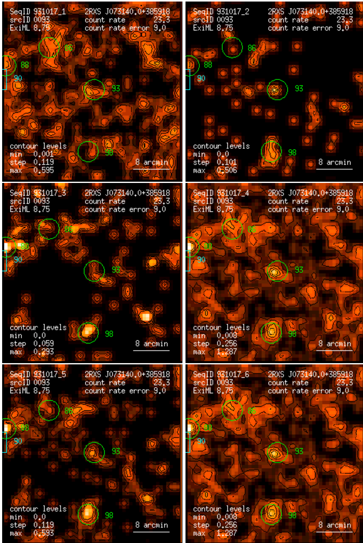
Figure 93: RASS 931017: detection 0093: band rate images, Gaussian filter: (1) PSPC channels 11 – 41, (2) 52 – 90, (3) 91 – 201, (4) 11 – 235, (5) 52 – 201, (6) 11 – 201. Broad band rates in counts/ks. Band rate contour levels in counts/ks/arcmin 2 .
