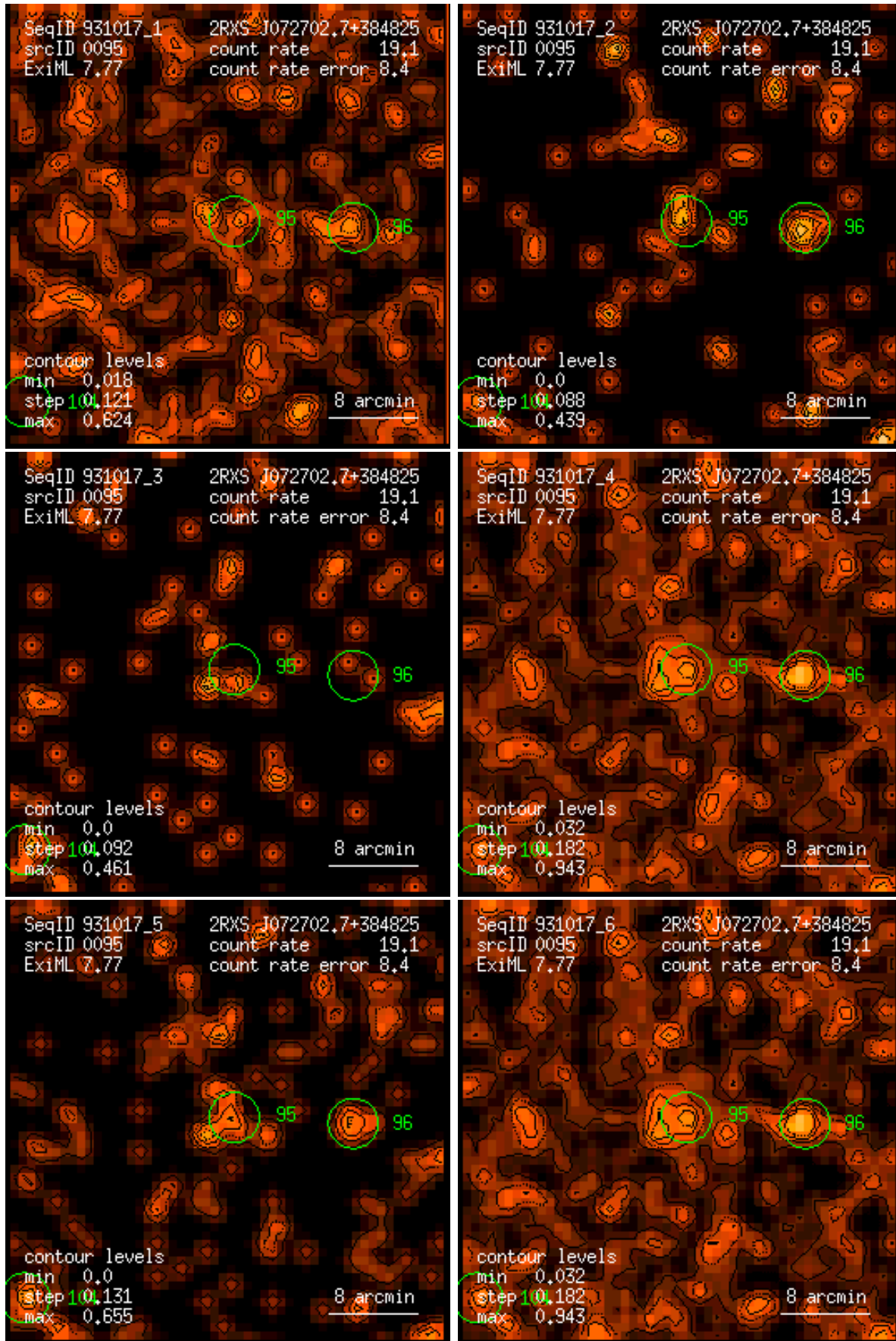
Figure 95: RASS 931017: detection 0095: band rate images, Gaussian filter: (1) PSPC channels 11 – 41, (2) 52 – 90, (3) 91 – 201, (4) 11 – 235, (5) 52 – 201, (6) 11 – 201. Broad band rates in counts/ks. Band rate contour levels in counts/ks/arcmin 2 .
