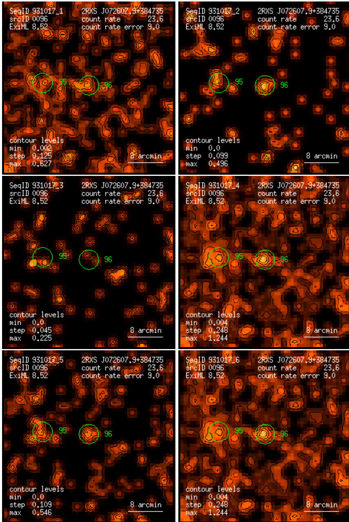
Figure 96: RASS 931017: detection 0096: band rate images, Gaussian filter: (1) PSPC channels 11 – 41, (2) 52 – 90, (3) 91 – 201, (4) 11 – 235, (5) 52 – 201, (6) 11 – 201. Broad band rates in counts/ks. Band rate contour levels in counts/ks/arcmin 2 .
