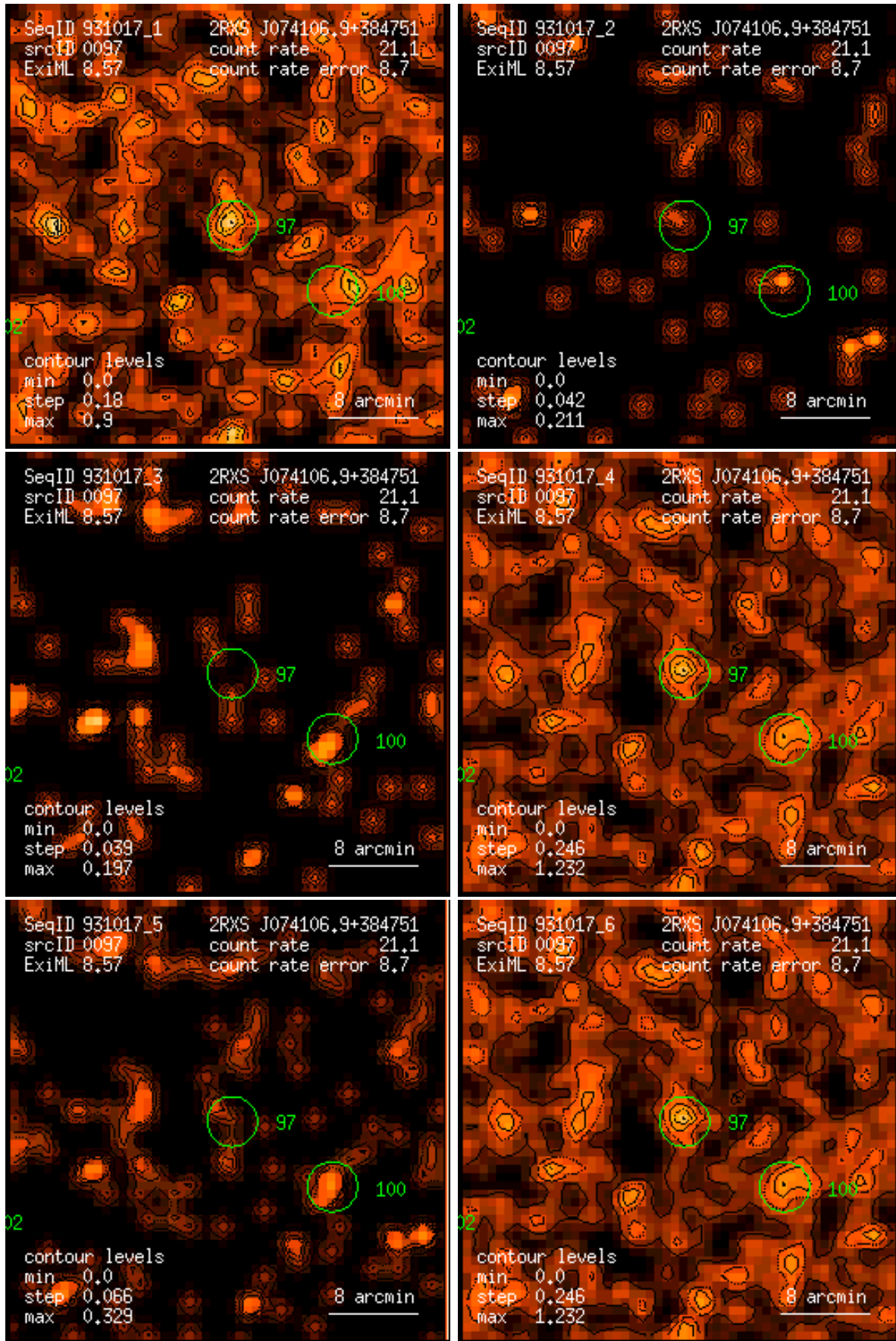
Figure 97: RASS 931017: detection 0097: band rate images, Gaussian filter: (1) PSPC channels 11 – 41, (2) 52 – 90, (3) 91 – 201, (4) 11 – 235, (5) 52 – 201, (6) 11 – 201. Broad band rates in counts/ks. Band rate contour levels in counts/ks/arcmin 2 .
