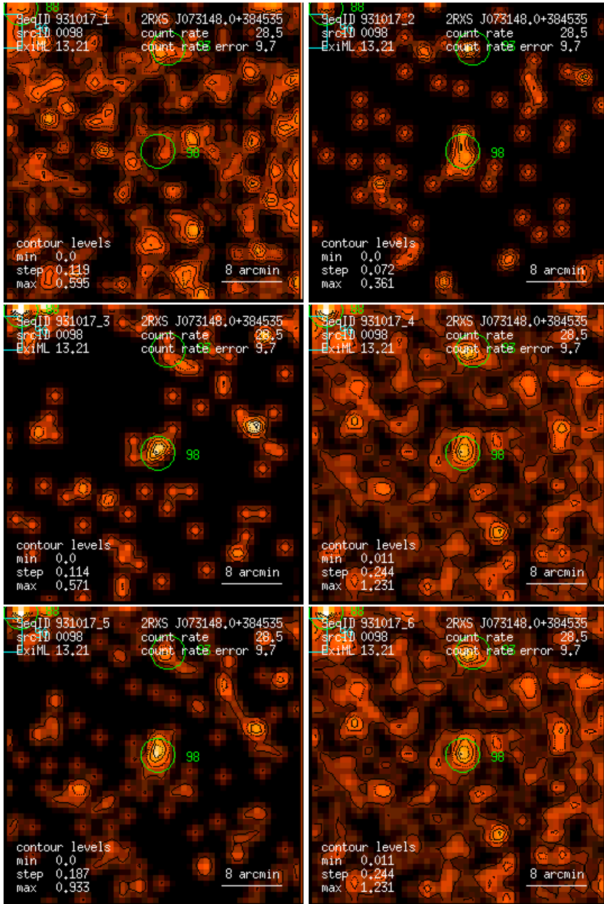
Figure 98: RASS 931017: detection 0098: band rate images, Gaussian filter: (1) PSPC channels 11 – 41, (2) 52 – 90, (3) 91 – 201, (4) 11 – 235, (5) 52 – 201, (6) 11 – 201. Broad band rates in counts/ks. Band rate contour levels in counts/ks/arcmin 2 .
