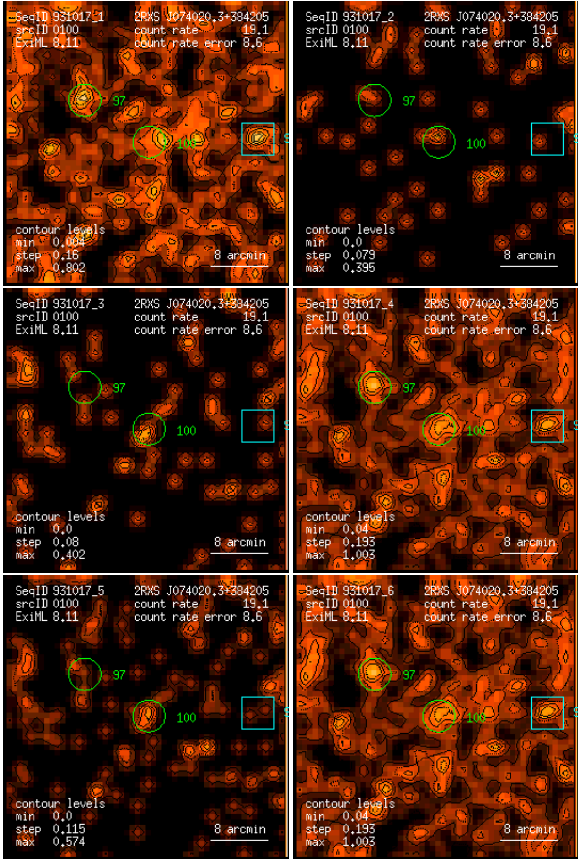
Figure 100: RASS 931017: detection 0100: band rate images, Gaussian filter: (1) PSPC channels 11 – 41, (2) 52 – 90, (3) 91 – 201, (4) 11 – 235, (5) 52 – 201, (6) 11 – 201. Broad band rates in counts/ks. Band rate contour levels in counts/ks/arcmin 2 .
