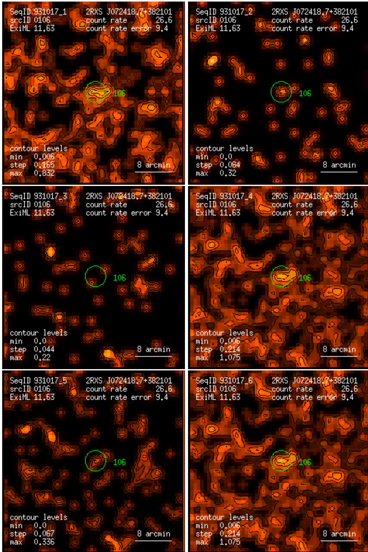
Figure 106: RASS 931017: detection 0106: band rate images, Gaussian filter: (1) PSPC channels 11 – 41, (2) 52 – 90, (3) 91 – 201, (4) 11 – 235, (5) 52 – 201, (6) 11 – 201. Broad band rates in counts/ks. Band rate contour levels in counts/ks/arcmin 2 .
