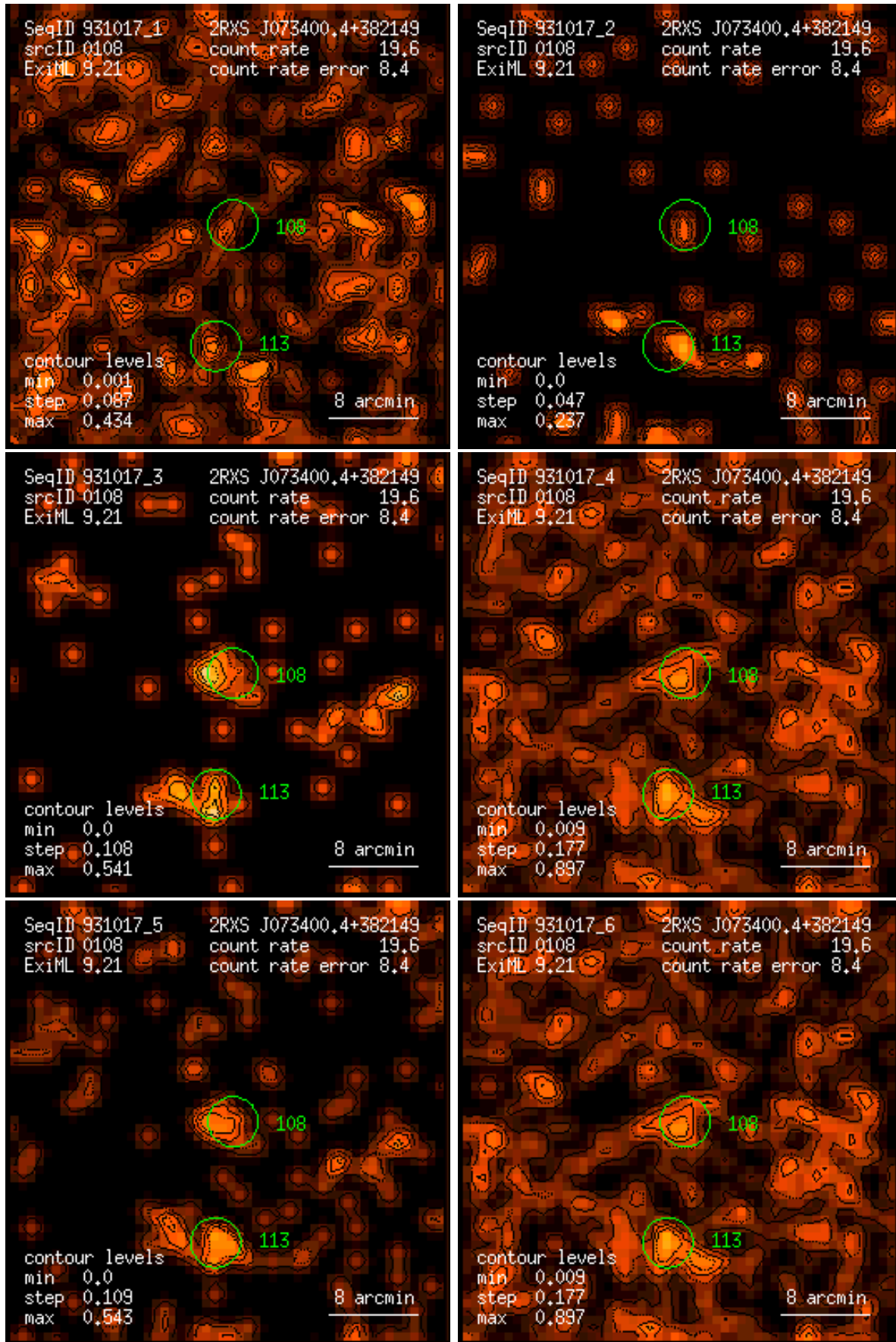
Figure 108: RASS 931017: detection 0108: band rate images, Gaussian filter: (1) PSPC channels 11 – 41, (2) 52 – 90, (3) 91 – 201, (4) 11 – 235, (5) 52 – 201, (6) 11 – 201. Broad band rates in counts/ks. Band rate contour levels in counts/ks/arcmin 2 .
