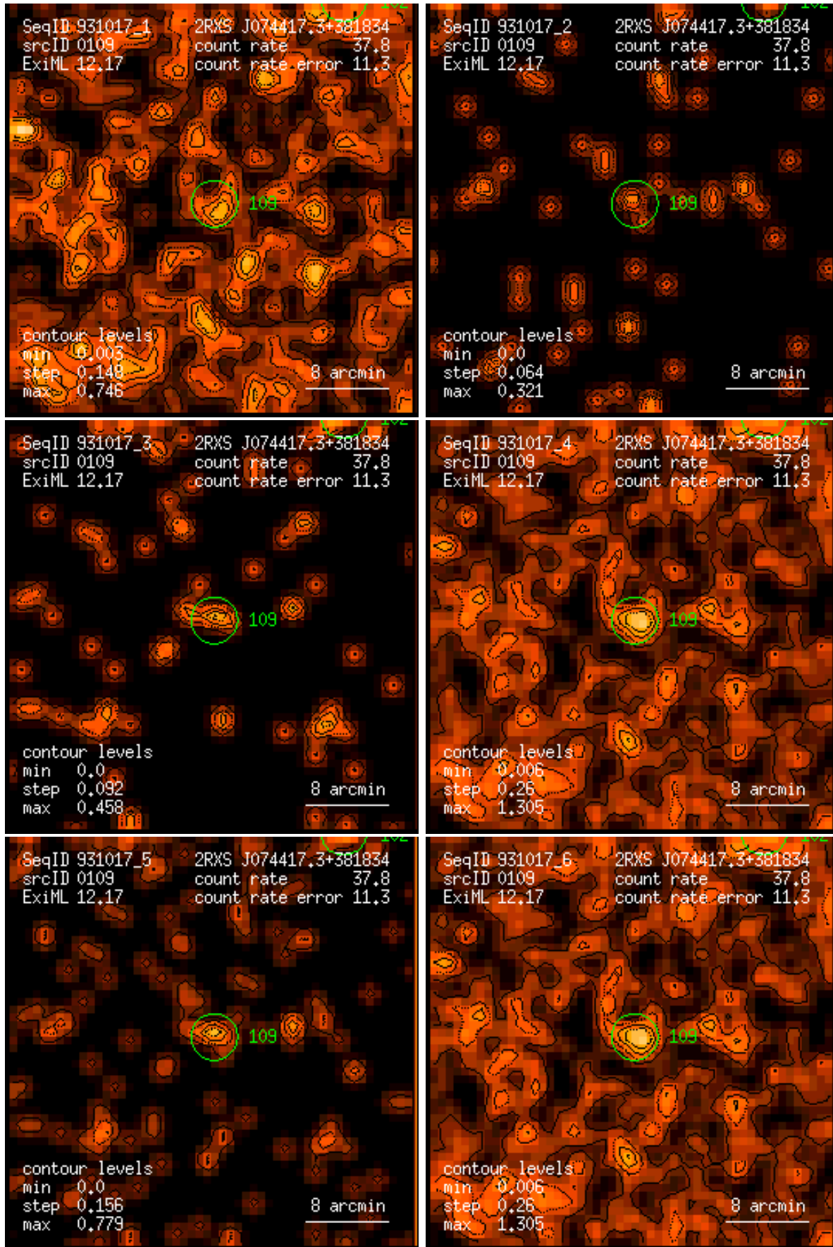
Figure 109: RASS 931017: detection 0109: band rate images, Gaussian filter: (1) PSPC channels 11 – 41, (2) 52 – 90, (3) 91 – 201, (4) 11 – 235, (5) 52 – 201, (6) 11 – 201. Broad band rates in counts/ks. Band rate contour levels in counts/ks/arcmin 2 .
