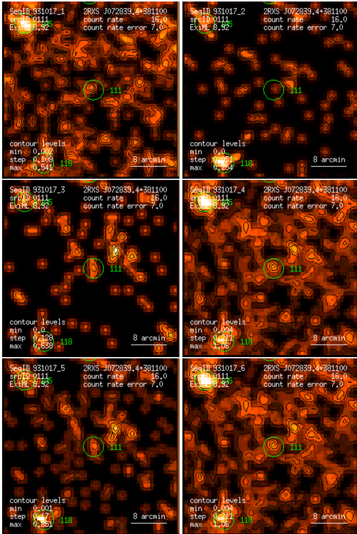
Figure 111: RASS 931017: detection 0111: band rate images, Gaussian filter: (1) PSPC channels 11 – 41, (2) 52 – 90, (3) 91 – 201, (4) 11 – 235, (5) 52 – 201, (6) 11 – 201. Broad band rates in counts/ks. Band rate contour levels in counts/ks/arcmin 2 .
