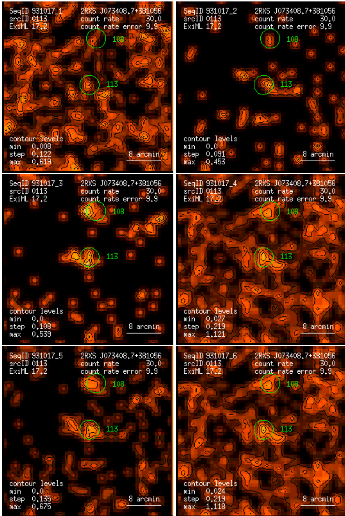
Figure 113: RASS 931017: detection 0113: band rate images, Gaussian filter: (1) PSPC channels 11 – 41, (2) 52 – 90, (3) 91 – 201, (4) 11 – 235, (5) 52 – 201, (6) 11 – 201. Broad band rates in counts/ks. Band rate contour levels in counts/ks/arcmin 2 .
