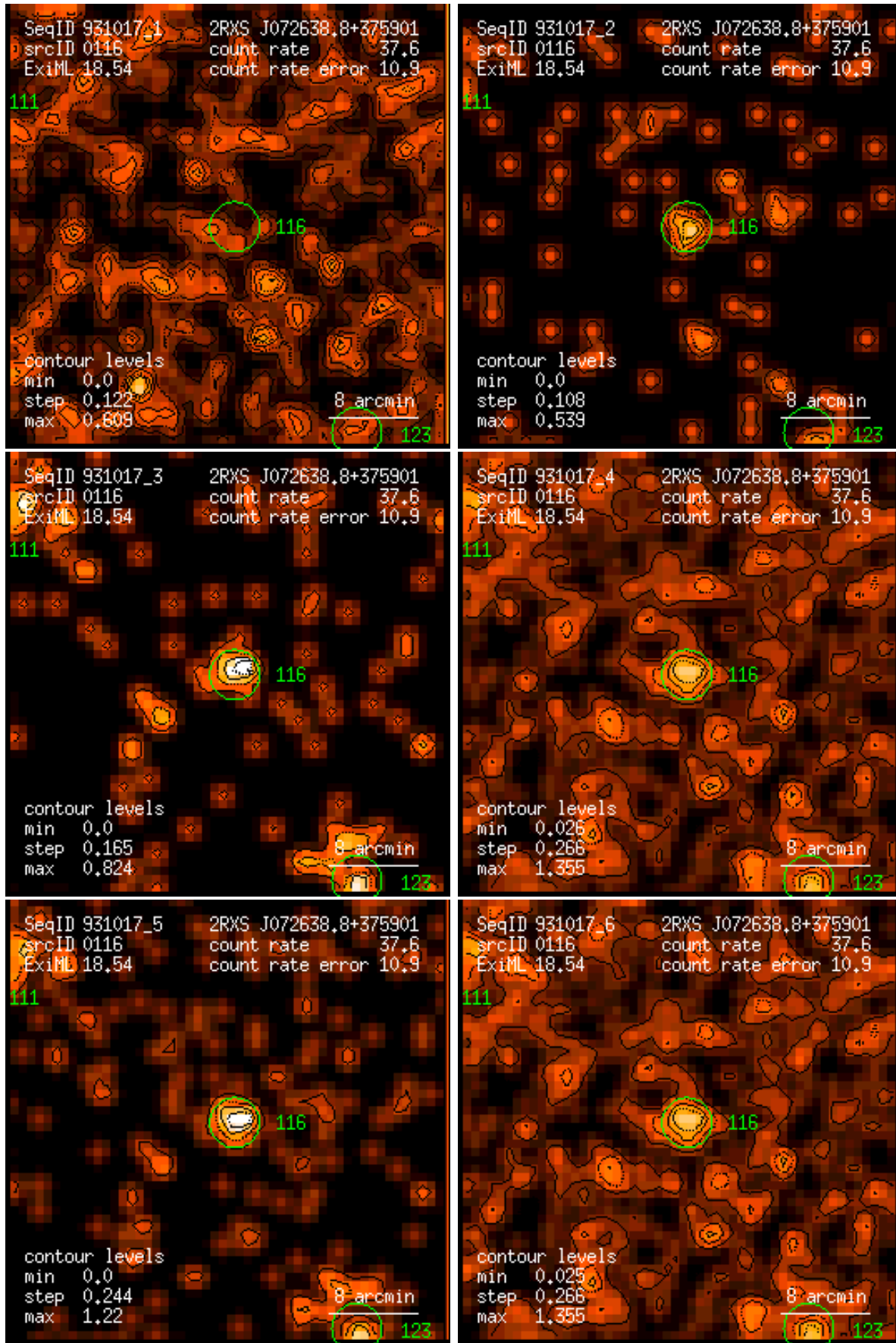
Figure 116: RASS 931017: detection 0116: band rate images, Gaussian filter: (1) PSPC channels 11 – 41, (2) 52 – 90, (3) 91 – 201, (4) 11 – 235, (5) 52 – 201, (6) 11 – 201. Broad band rates in counts/ks. Band rate contour levels in counts/ks/arcmin 2 .
