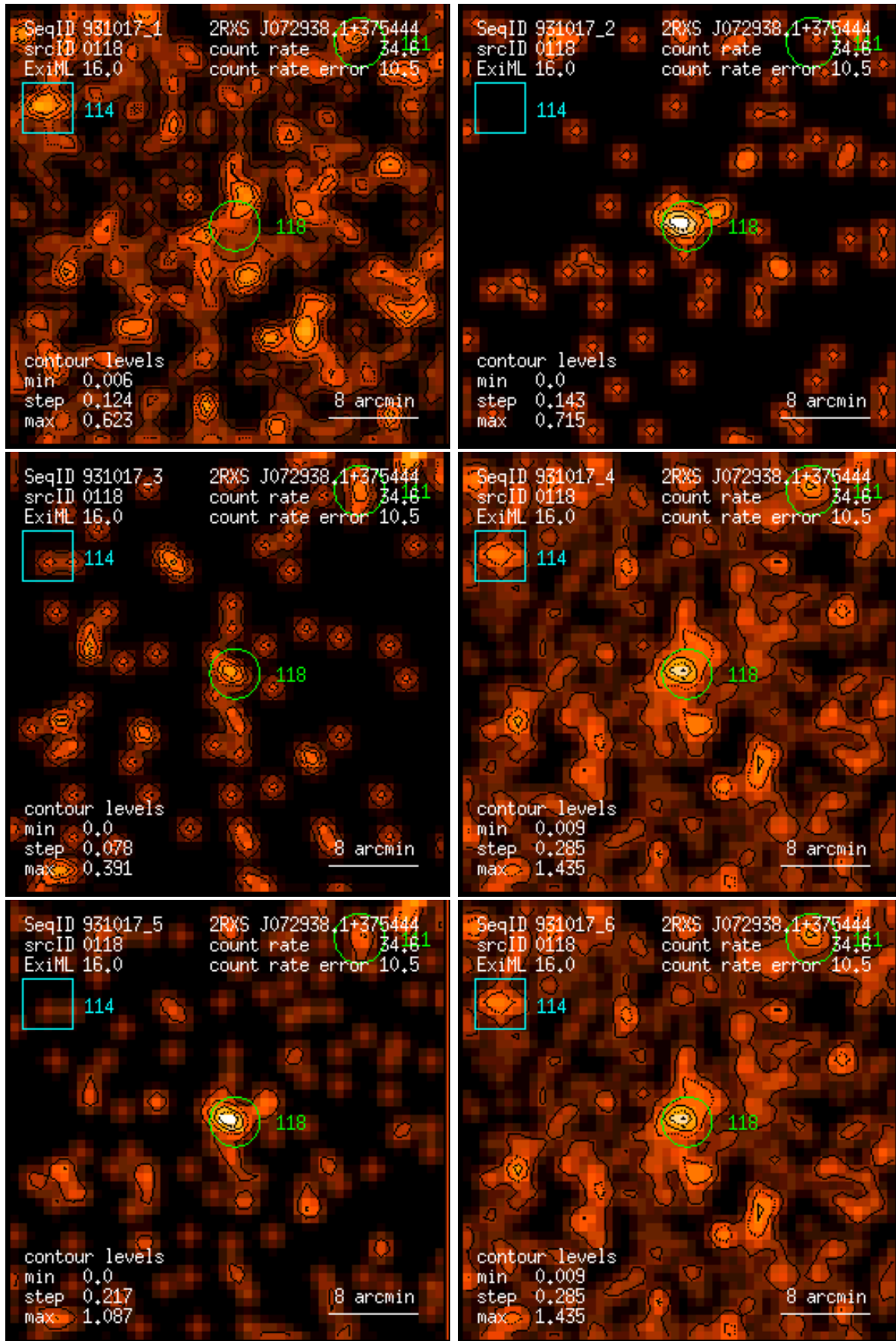
Figure 118: RASS 931017: detection 0118: band rate images, Gaussian filter: (1) PSPC channels 11 – 41, (2) 52 – 90, (3) 91 – 201, (4) 11 – 235, (5) 52 – 201, (6) 11 – 201. Broad band rates in counts/ks. Band rate contour levels in counts/ks/arcmin 2 .
