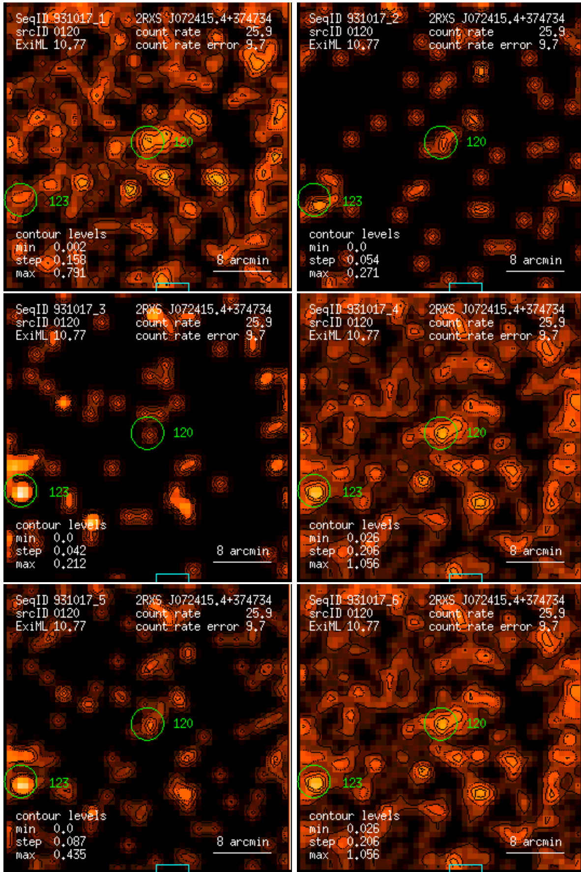
Figure 120: RASS 931017: detection 0120: band rate images, Gaussian filter: (1) PSPC channels 11 – 41, (2) 52 – 90, (3) 91 – 201, (4) 11 – 235, (5) 52 – 201, (6) 11 – 201. Broad band rates in counts/ks. Band rate contour levels in counts/ks/arcmin 2 .
