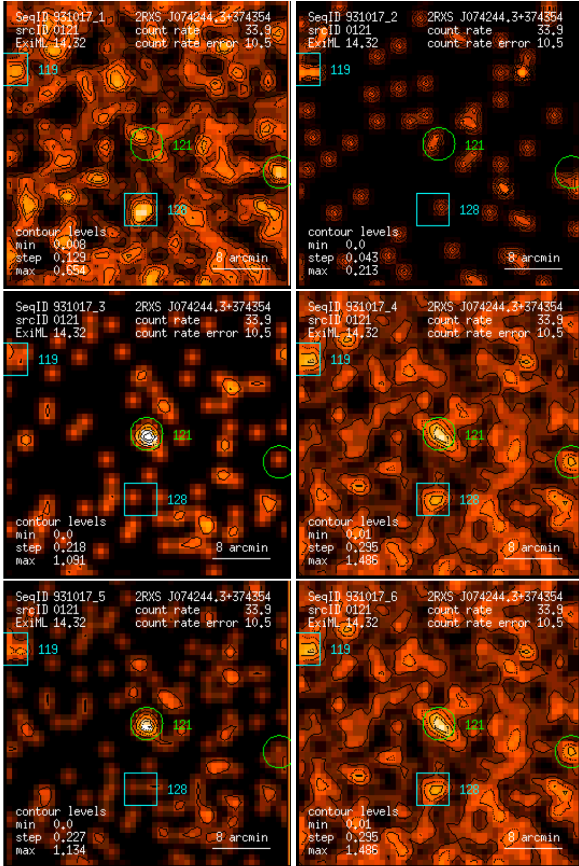
Figure 121: RASS 931017: detection 0121: band rate images, Gaussian filter: (1) PSPC channels 11 – 41, (2) 52 – 90, (3) 91 – 201, (4) 11 – 235, (5) 52 – 201, (6) 11 – 201. Broad band rates in counts/ks. Band rate contour levels in counts/ks/arcmin 2 .
