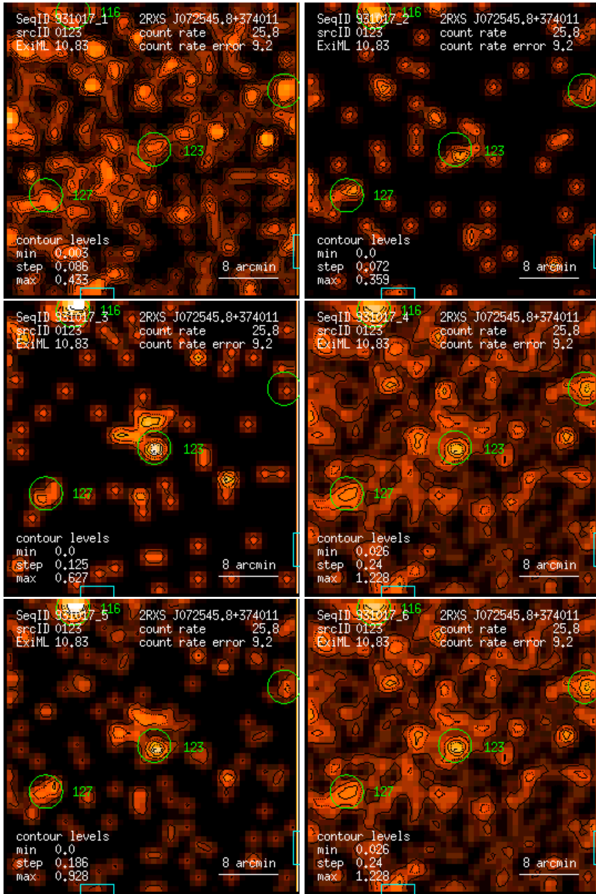
Figure 123: RASS 931017: detection 0123: band rate images, Gaussian filter: (1) PSPC channels 11 – 41, (2) 52 – 90, (3) 91 – 201, (4) 11 – 235, (5) 52 – 201, (6) 11 – 201. Broad band rates in counts/ks. Band rate contour levels in counts/ks/arcmin 2 .
